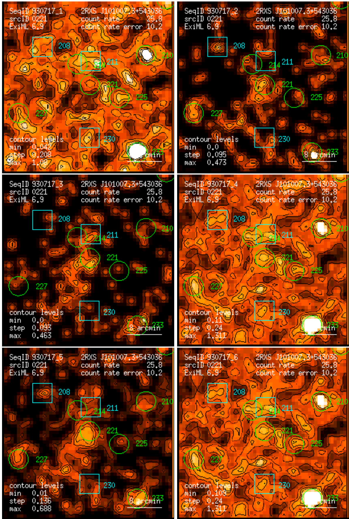
Figure 221: RASS 930717: detection 0221: band rate images, Gaussian filter: (1) PSPC channels 11 – 41, (2) 52 – 90, (3) 91 – 201, (4) 11 – 235, (5) 52 – 201, (6) 11 – 201. Broad band rates in counts/ks. Band rate contour levels in counts/ks/arcmin 2 .
