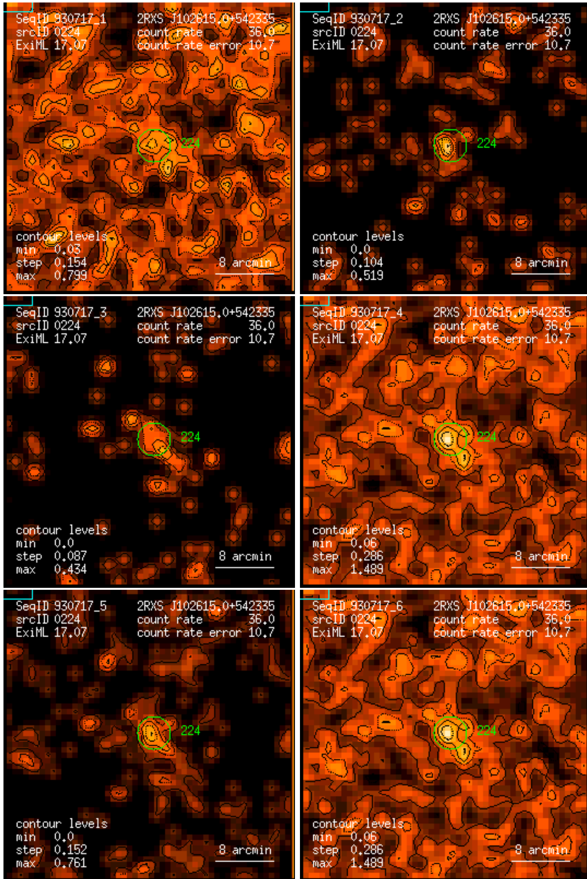
Figure 224: RASS 930717: detection 0224: band rate images, Gaussian filter: (1) PSPC channels 11 – 41, (2) 52 – 90, (3) 91 – 201, (4) 11 – 235, (5) 52 – 201, (6) 11 – 201. Broad band rates in counts/ks. Band rate contour levels in counts/ks/arcmin 2 .
