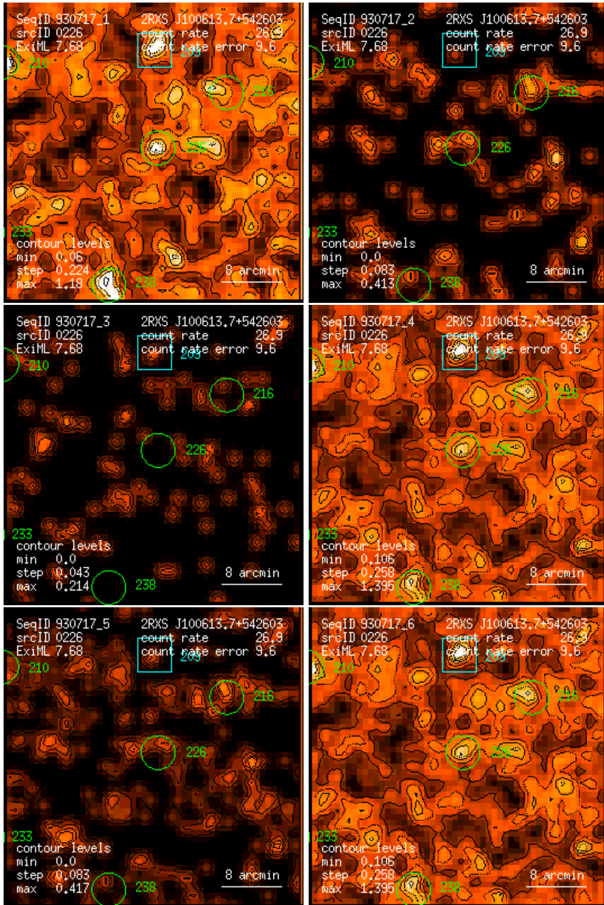
Figure 226: RASS 930717: detection 0226: band rate images, Gaussian filter: (1) PSPC channels 11 – 41, (2) 52 – 90, (3) 91 – 201, (4) 11 – 235, (5) 52 – 201, (6) 11 – 201. Broad band rates in counts/ks. Band rate contour levels in counts/ks/arcmin 2 .
