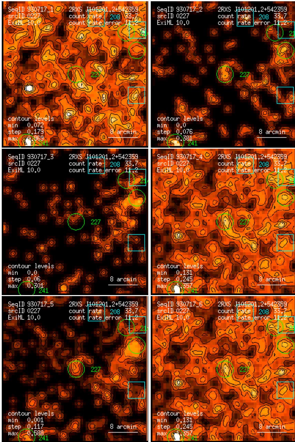
Figure 227: RASS 930717: detection 0227: band rate images, Gaussian filter: (1) PSPC channels 11 – 41, (2) 52 – 90, (3) 91 – 201, (4) 11 – 235, (5) 52 – 201, (6) 11 – 201. Broad band rates in counts/ks. Band rate contour levels in counts/ks/arcmin 2 .
