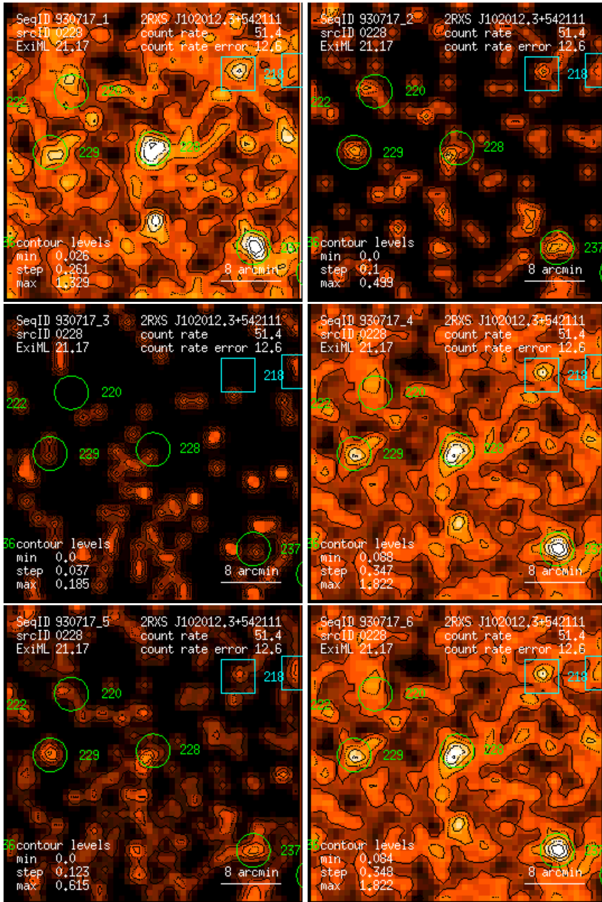
Figure 228: RASS 930717: detection 0228: band rate images, Gaussian filter: (1) PSPC channels 11 – 41, (2) 52 – 90, (3) 91 – 201, (4) 11 – 235, (5) 52 – 201, (6) 11 – 201. Broad band rates in counts/ks. Band rate contour levels in counts/ks/arcmin 2 .
