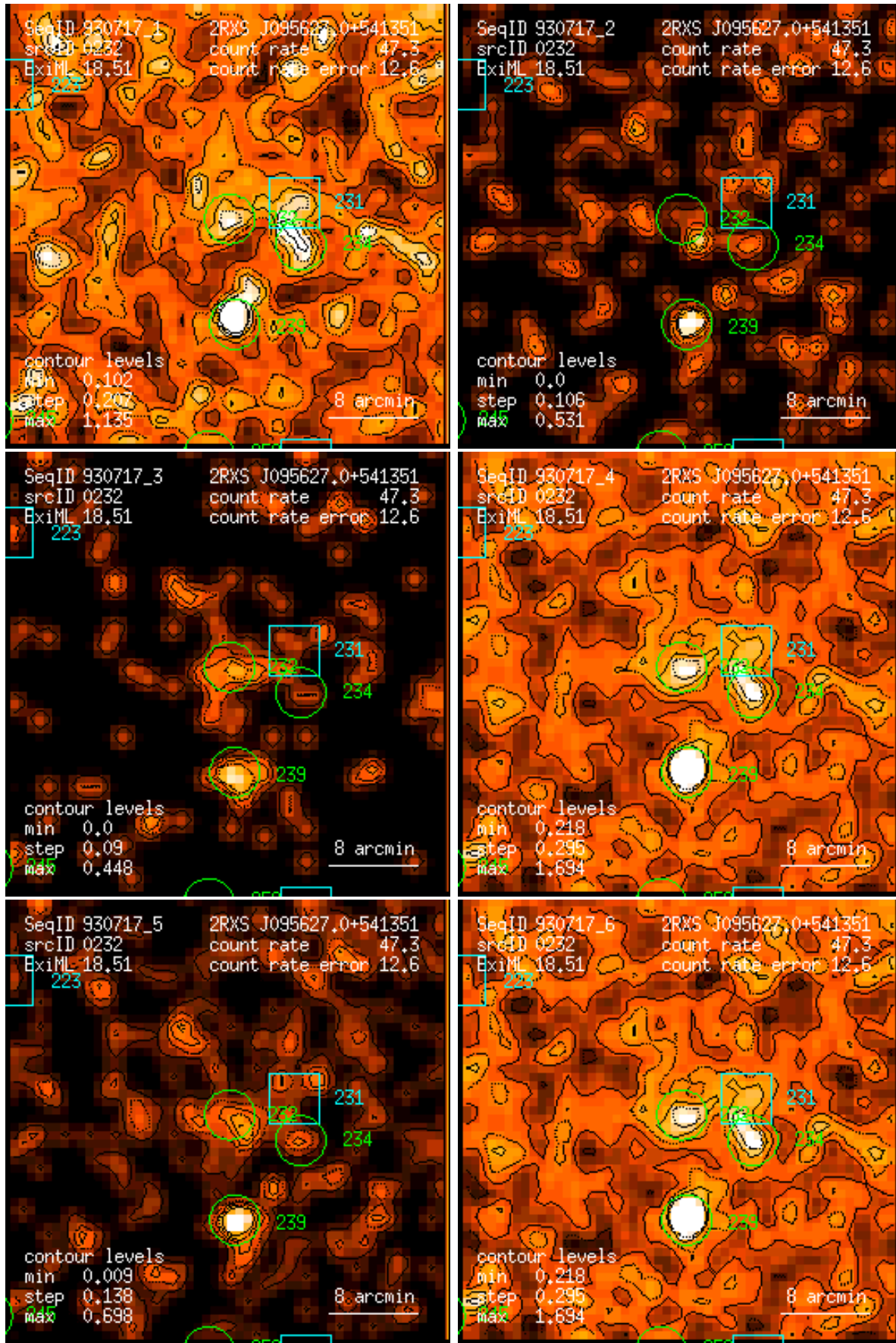
Figure 232: RASS 930717: detection 0232: band rate images, Gaussian filter: (1) PSPC channels 11 – 41, (2) 52 – 90, (3) 91 – 201, (4) 11 – 235, (5) 52 – 201, (6) 11 – 201. Broad band rates in counts/ks. Band rate contour levels in counts/ks/arcmin 2 .
