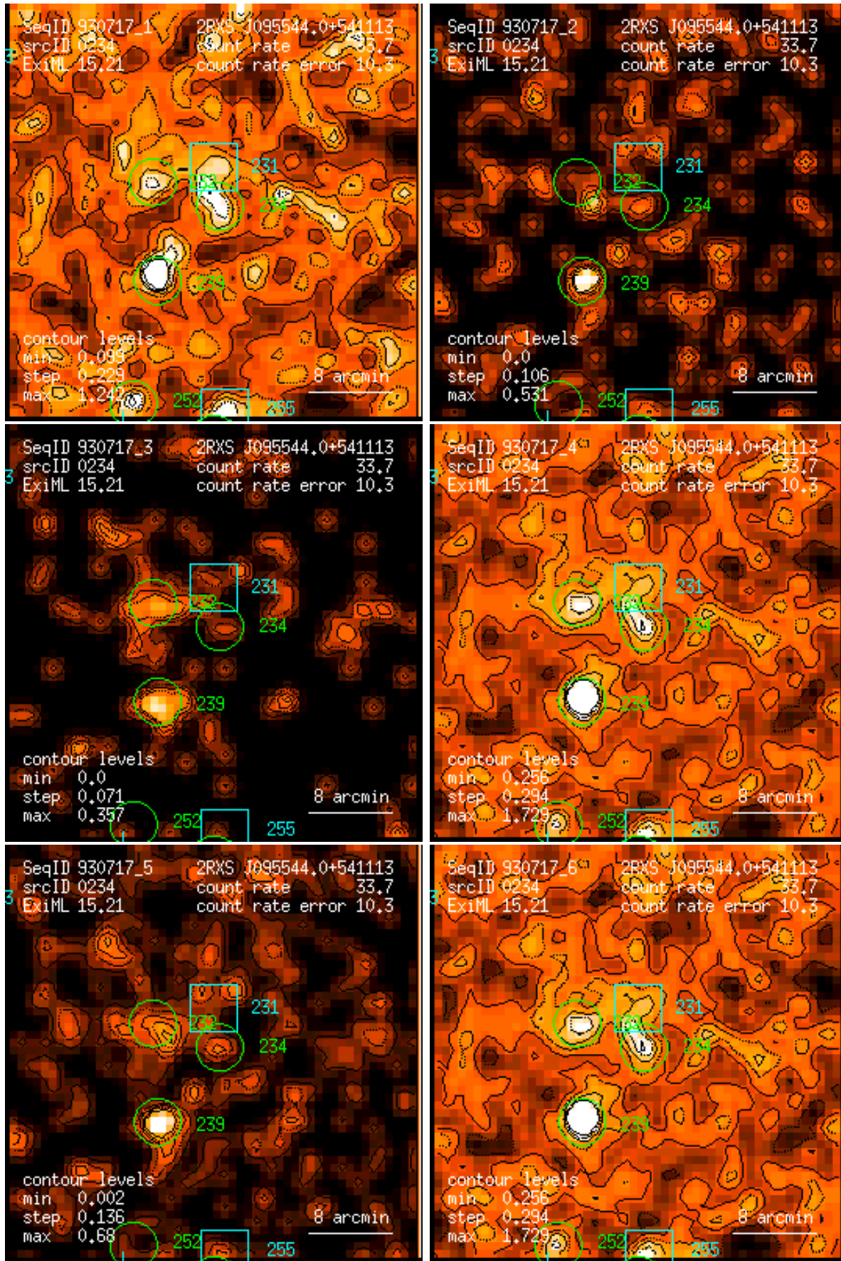
Figure 234: RASS 930717: detection 0234: band rate images, Gaussian filter: (1) PSPC channels 11 – 41, (2) 52 – 90, (3) 91 – 201, (4) 11 – 235, (5) 52 – 201, (6) 11 – 201. Broad band rates in counts/ks. Band rate contour levels in counts/ks/arcmin 2 .
