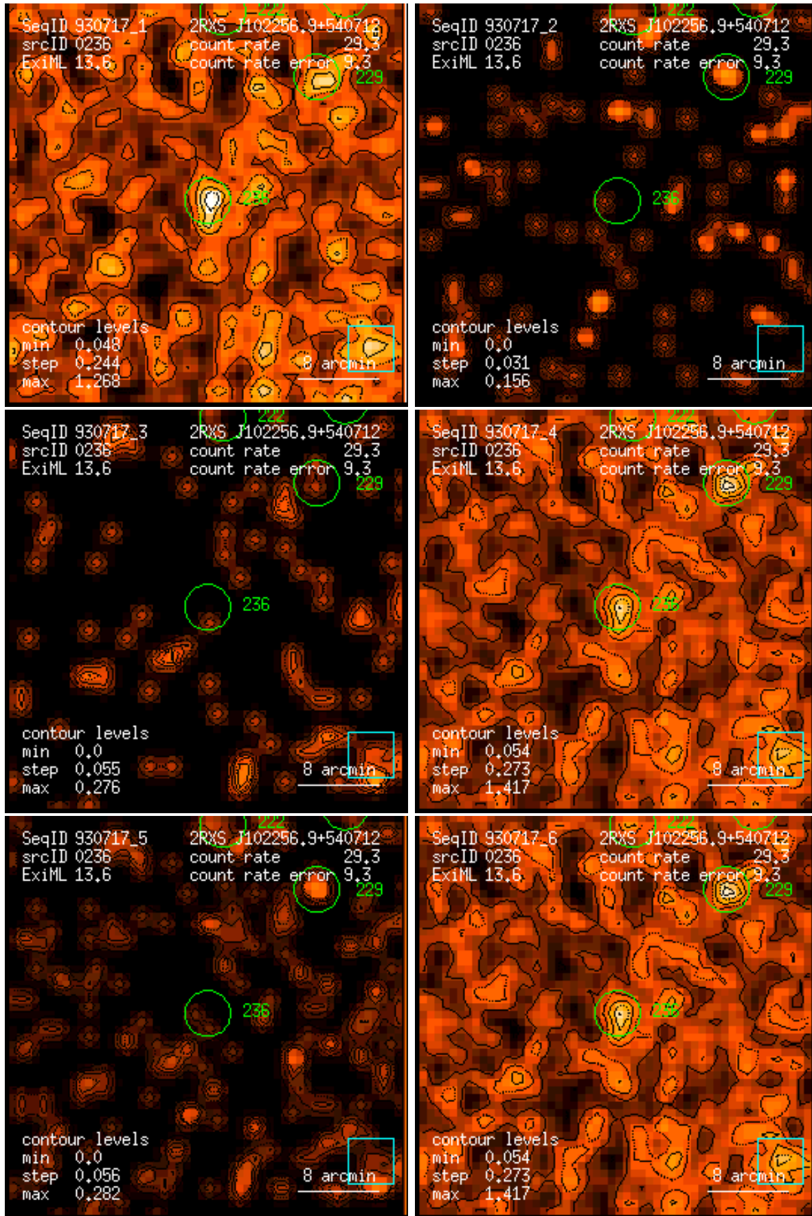
Figure 236: RASS 930717: detection 0236: band rate images, Gaussian filter: (1) PSPC channels 11 – 41, (2) 52 – 90, (3) 91 – 201, (4) 11 – 235, (5) 52 – 201, (6) 11 – 201. Broad band rates in counts/ks. Band rate contour levels in counts/ks/arcmin 2 .
