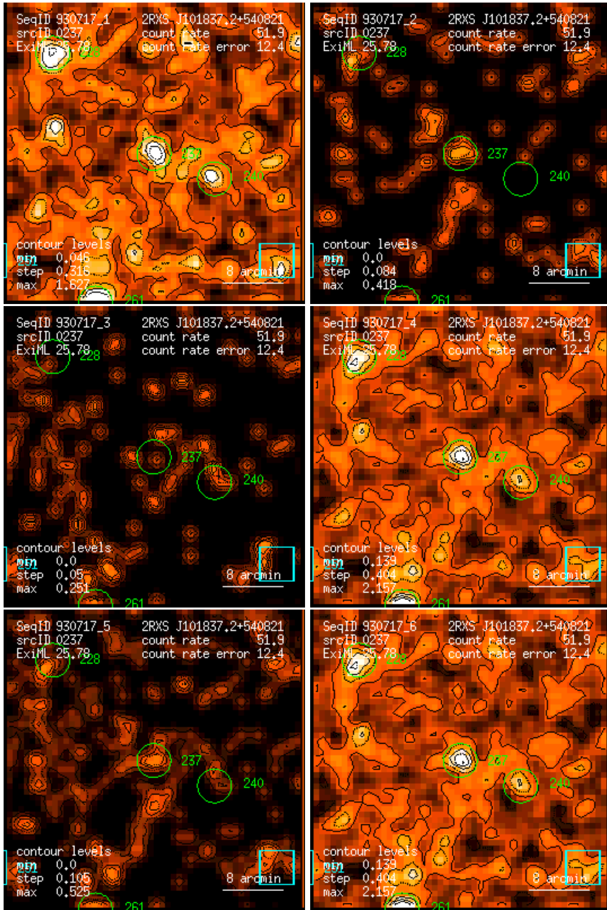
Figure 237: RASS 930717: detection 0237: band rate images, Gaussian filter: (1) PSPC channels 11 – 41, (2) 52 – 90, (3) 91 – 201, (4) 11 – 235, (5) 52 – 201, (6) 11 – 201. Broad band rates in counts/ks. Band rate contour levels in counts/ks/arcmin 2 .
