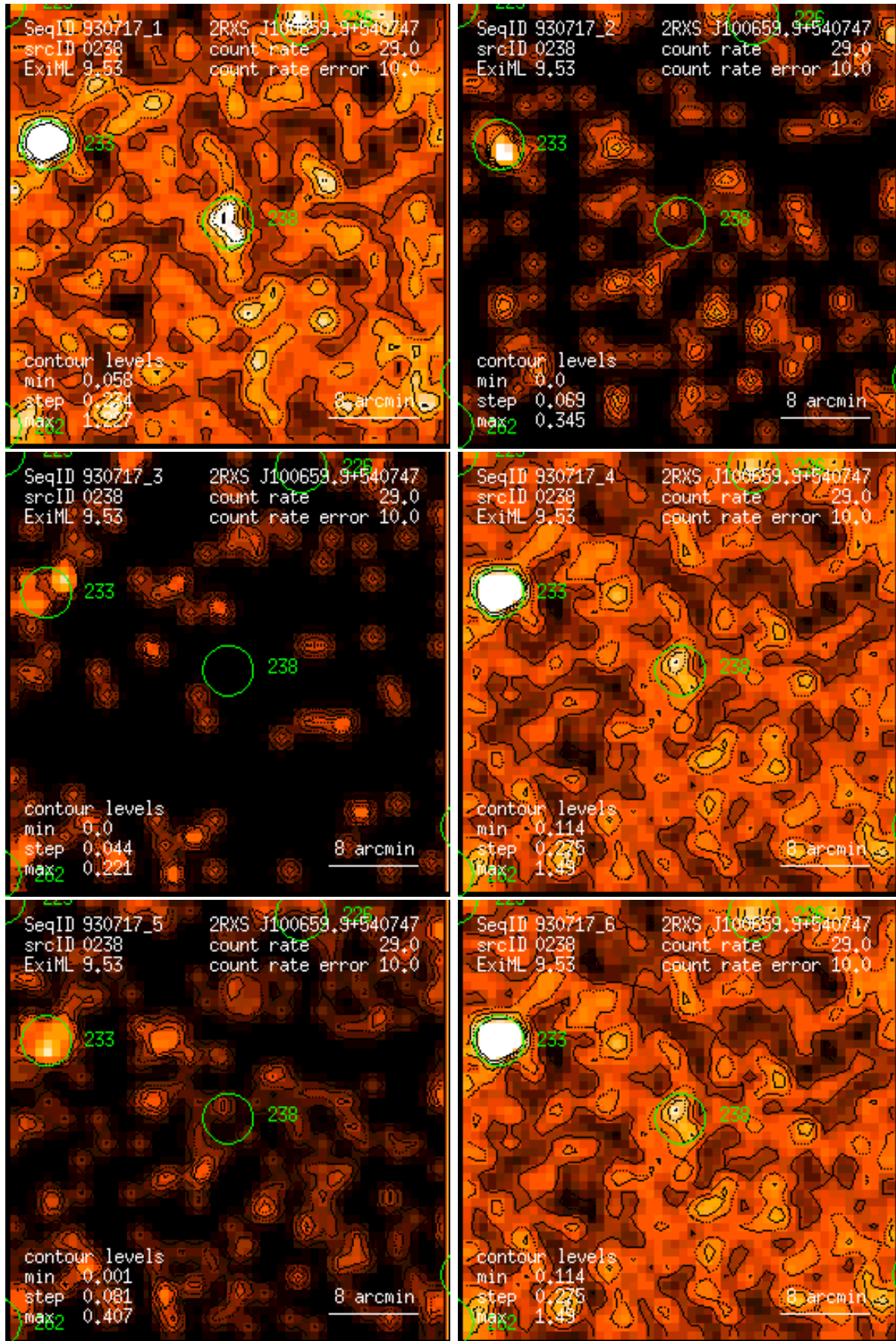
Figure 238: RASS 930717: detection 0238: band rate images, Gaussian filter: (1) PSPC channels 11 – 41, (2) 52 – 90, (3) 91 – 201, (4) 11 – 235, (5) 52 – 201, (6) 11 – 201. Broad band rates in counts/ks. Band rate contour levels in counts/ks/arcmin 2 .
