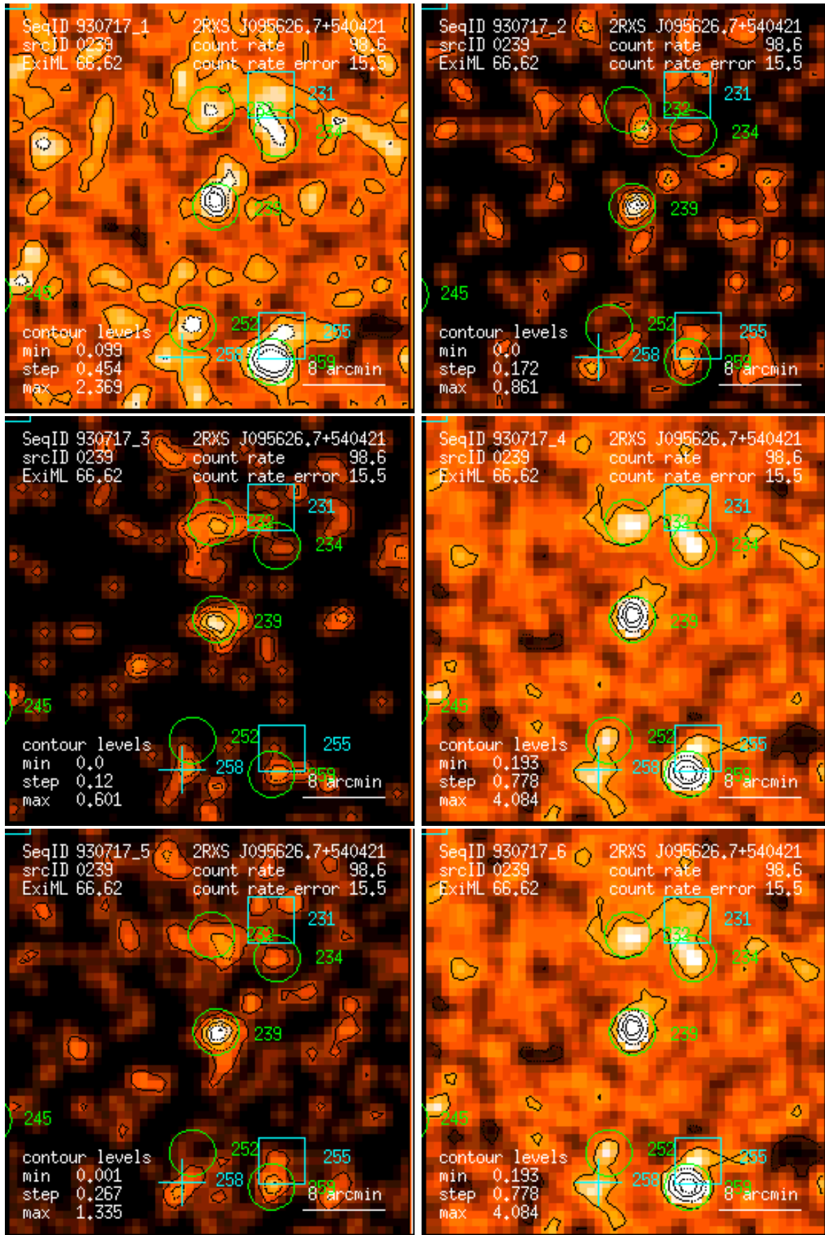
Figure 239: RASS 930717: detection 0239: band rate images, Gaussian filter: (1) PSPC channels 11 – 41, (2) 52 – 90, (3) 91 – 201, (4) 11 – 235, (5) 52 – 201, (6) 11 – 201. Broad band rates in counts/ks. Band rate contour levels in counts/ks/arcmin 2 .
