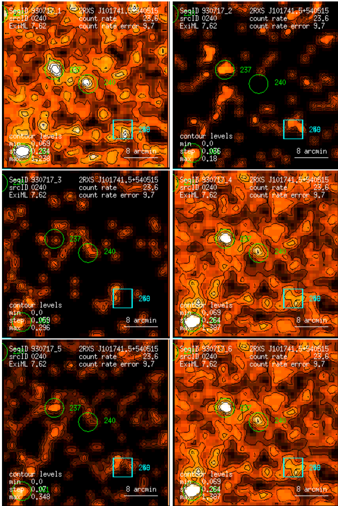
Figure 240: RASS 930717: detection 0240: band rate images, Gaussian filter: (1) PSPC channels 11 – 41, (2) 52 – 90, (3) 91 – 201, (4) 11 – 235, (5) 52 – 201, (6) 11 – 201. Broad band rates in counts/ks. Band rate contour levels in counts/ks/arcmin 2 .
