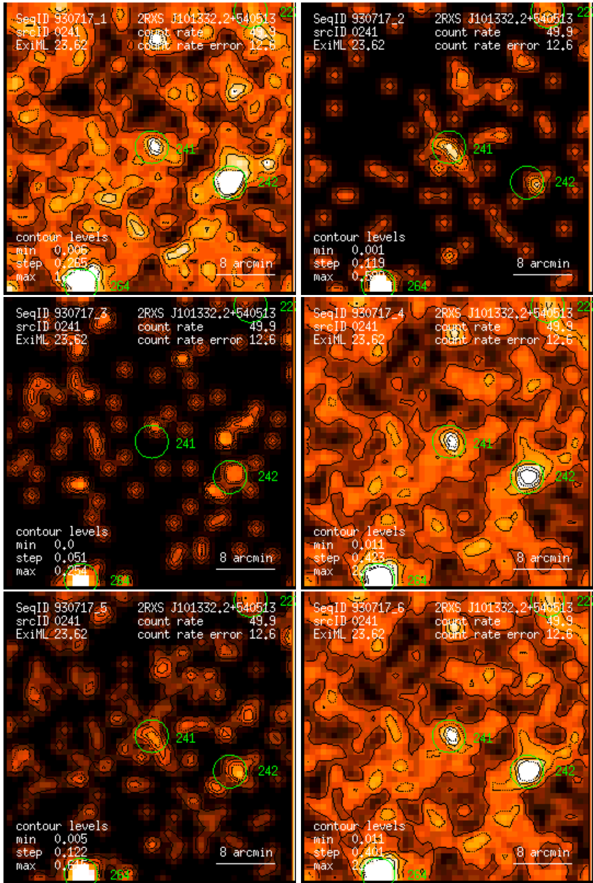
Figure 241: RASS 930717: detection 0241: band rate images, Gaussian filter: (1) PSPC channels 11 – 41, (2) 52 – 90, (3) 91 – 201, (4) 11 – 235, (5) 52 – 201, (6) 11 – 201. Broad band rates in counts/ks. Band rate contour levels in counts/ks/arcmin 2 .
