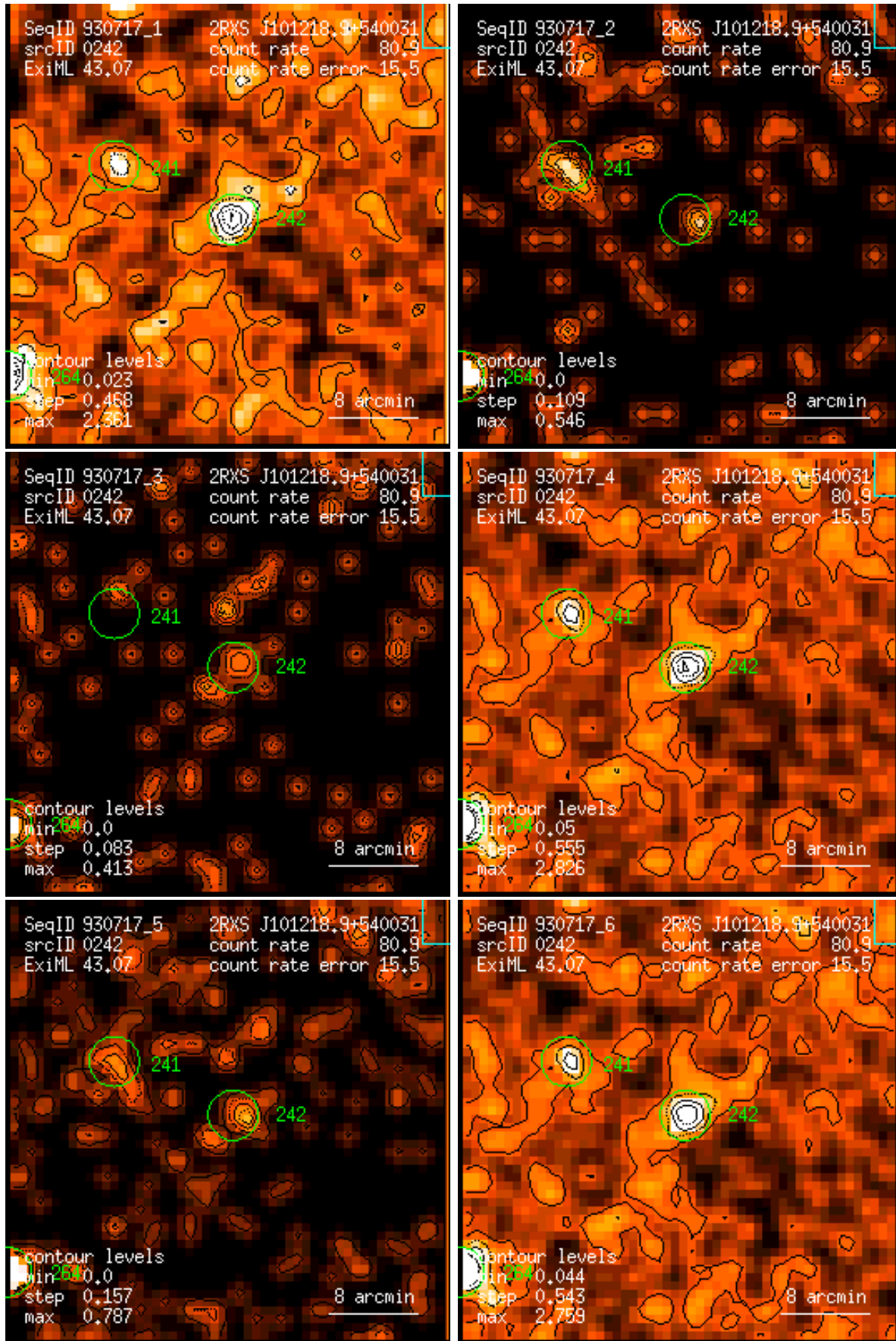
Figure 242: RASS 930717: detection 0242: band rate images, Gaussian filter: (1) PSPC channels 11 – 41, (2) 52 – 90, (3) 91 – 201, (4) 11 – 235, (5) 52 – 201, (6) 11 – 201. Broad band rates in counts/ks. Band rate contour levels in counts/ks/arcmin 2 .
