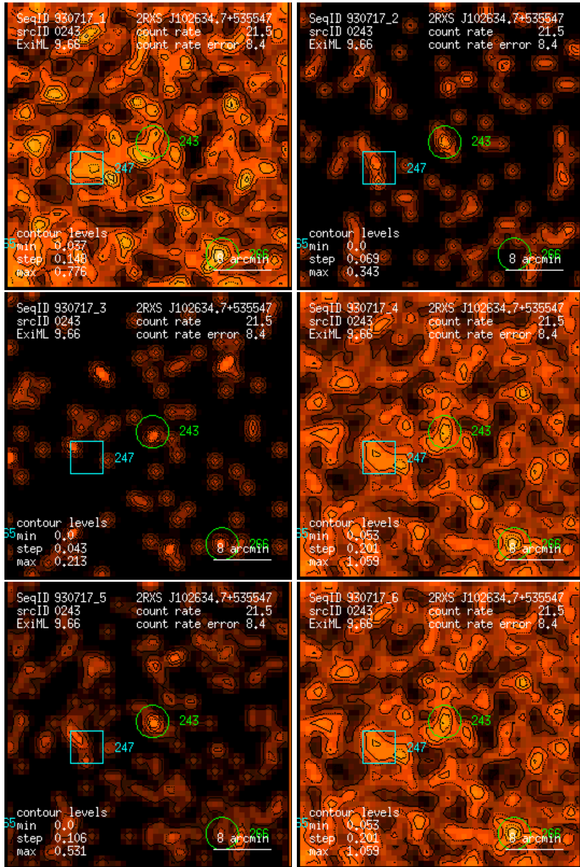
Figure 243: RASS 930717: detection 0243: band rate images, Gaussian filter: (1) PSPC channels 11 – 41, (2) 52 – 90, (3) 91 – 201, (4) 11 – 235, (5) 52 – 201, (6) 11 – 201. Broad band rates in counts/ks. Band rate contour levels in counts/ks/arcmin 2 .
