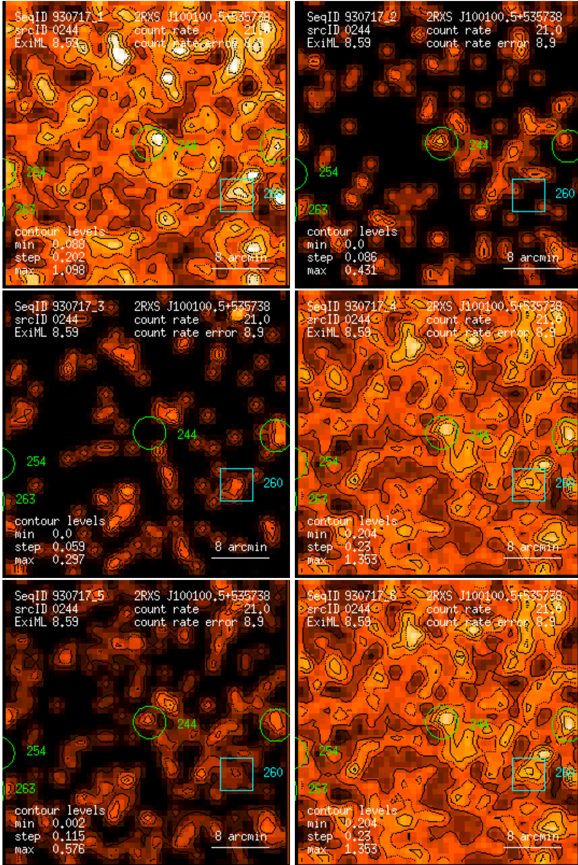
Figure 244: RASS 930717: detection 0244: band rate images, Gaussian filter: (1) PSPC channels 11 – 41, (2) 52 – 90, (3) 91 – 201, (4) 11 – 235, (5) 52 – 201, (6) 11 – 201. Broad band rates in counts/ks. Band rate contour levels in counts/ks/arcmin 2 .
