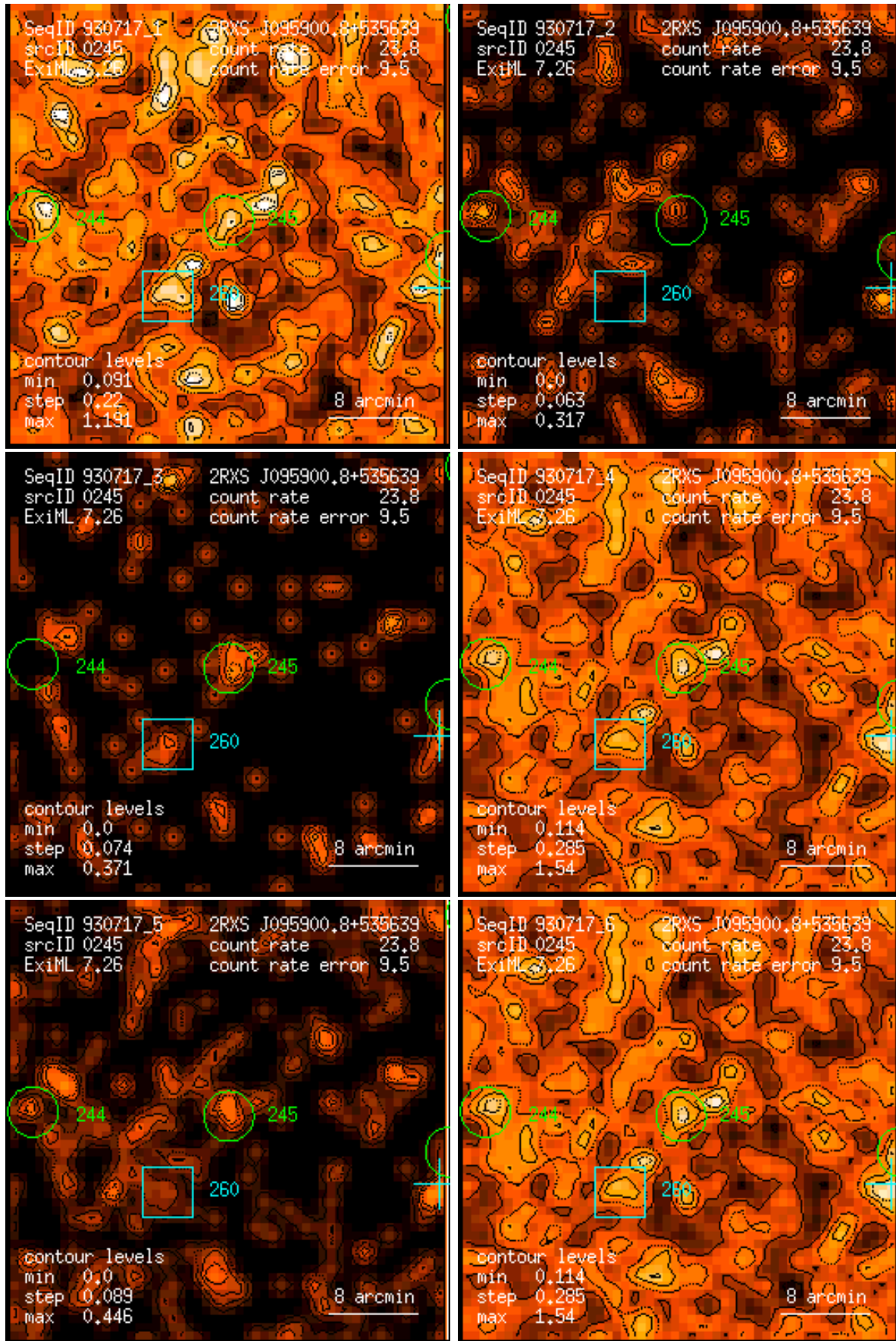
Figure 245: RASS 930717: detection 0245: band rate images, Gaussian filter: (1) PSPC channels 11 – 41, (2) 52 – 90, (3) 91 – 201, (4) 11 – 235, (5) 52 – 201, (6) 11 – 201. Broad band rates in counts/ks. Band rate contour levels in counts/ks/arcmin 2 .
