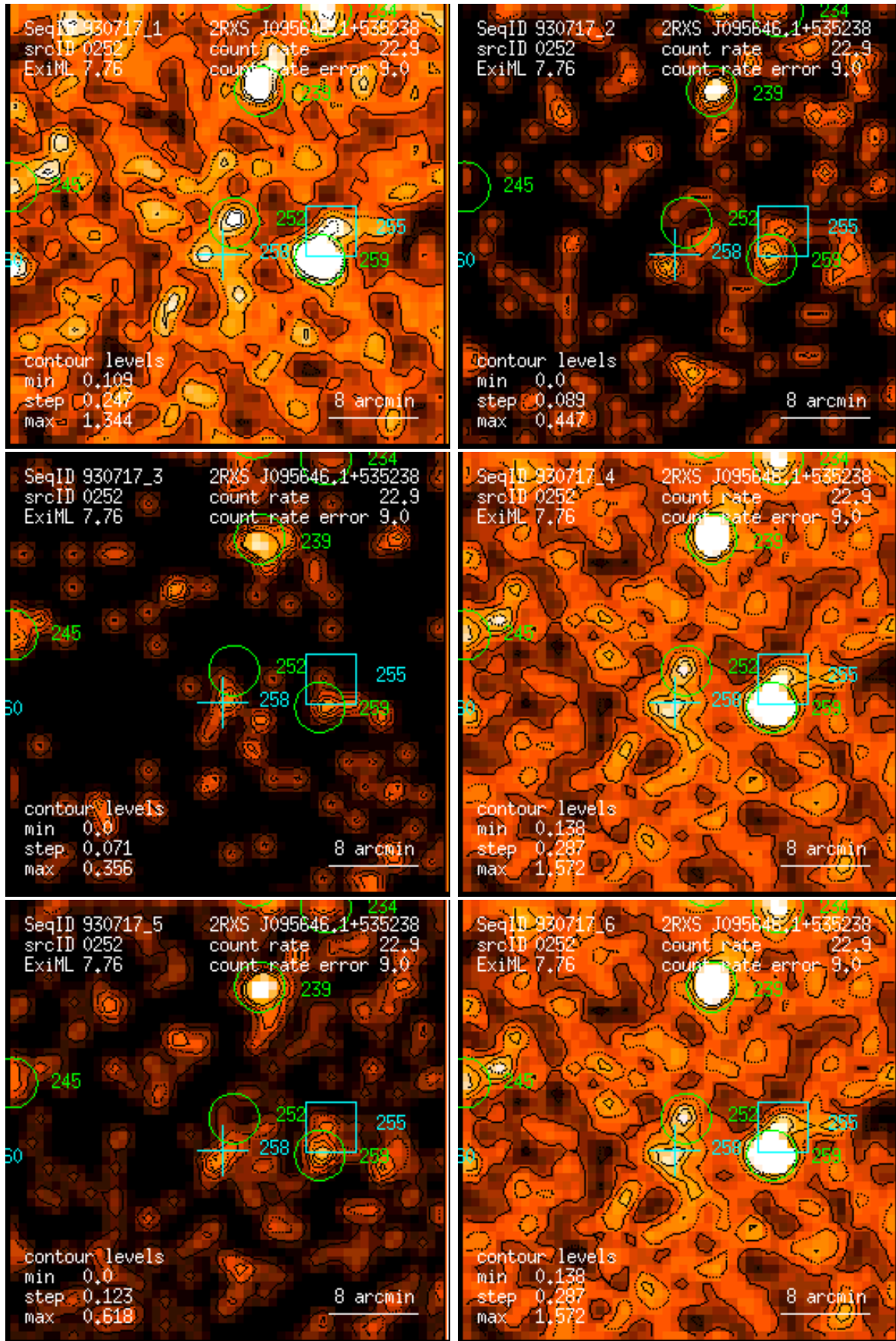
Figure 252: RASS 930717: detection 0252: band rate images, Gaussian filter: (1) PSPC channels 11 – 41, (2) 52 – 90, (3) 91 – 201, (4) 11 – 235, (5) 52 – 201, (6) 11 – 201. Broad band rates in counts/ks. Band rate contour levels in counts/ks/arcmin 2 .
