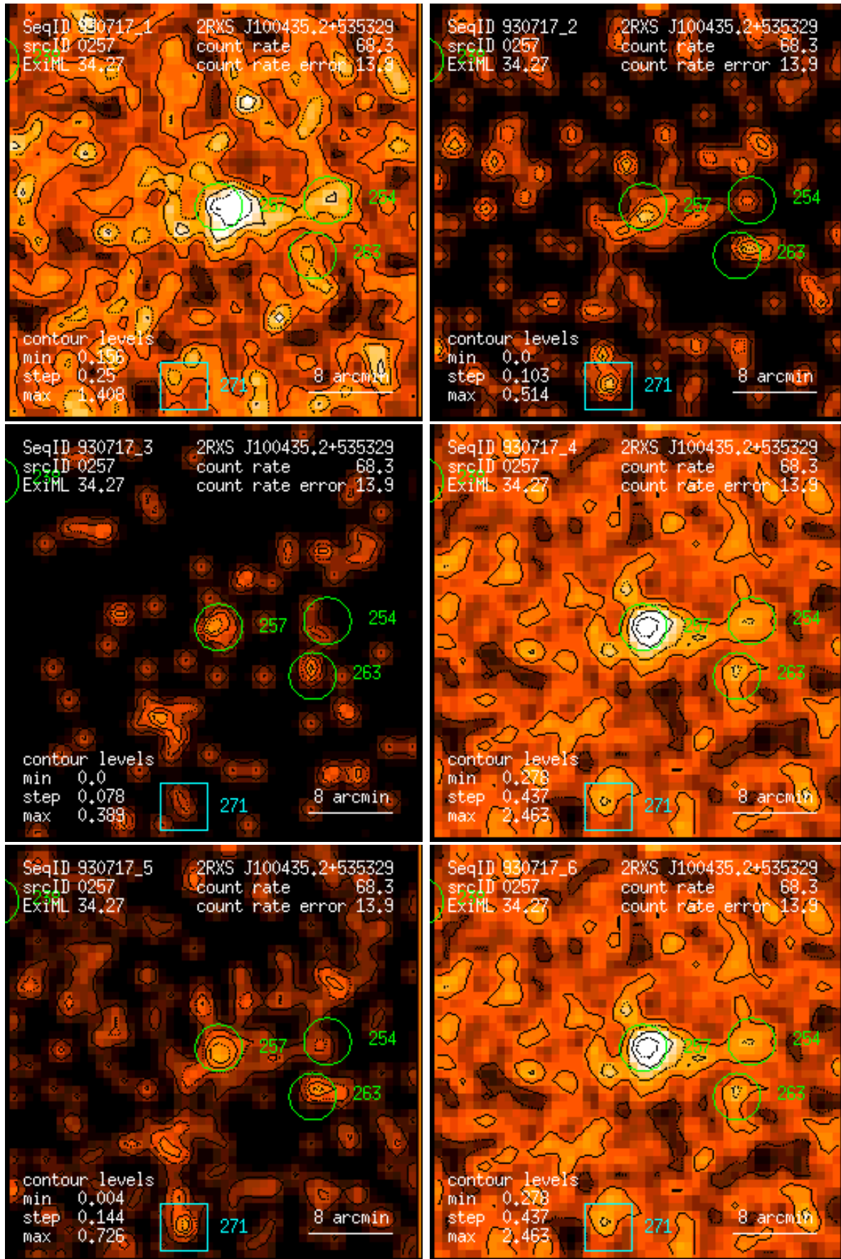
Figure 257: RASS 930717: detection 0257: band rate images, Gaussian filter: (1) PSPC channels 11 – 41, (2) 52 – 90, (3) 91 – 201, (4) 11 – 235, (5) 52 – 201, (6) 11 – 201. Broad band rates in counts/ks. Band rate contour levels in counts/ks/arcmin 2 .
