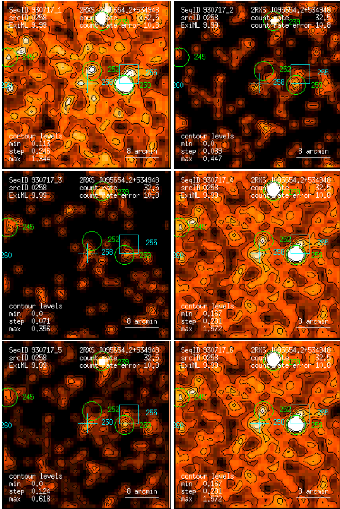
Figure 258: RASS 930717: detection 0258: band rate images, Gaussian filter: (1) PSPC channels 11 – 41, (2) 52 – 90, (3) 91 – 201, (4) 11 – 235, (5) 52 – 201, (6) 11 – 201. Broad band rates in counts/ks. Band rate contour levels in counts/ks/arcmin 2 .
