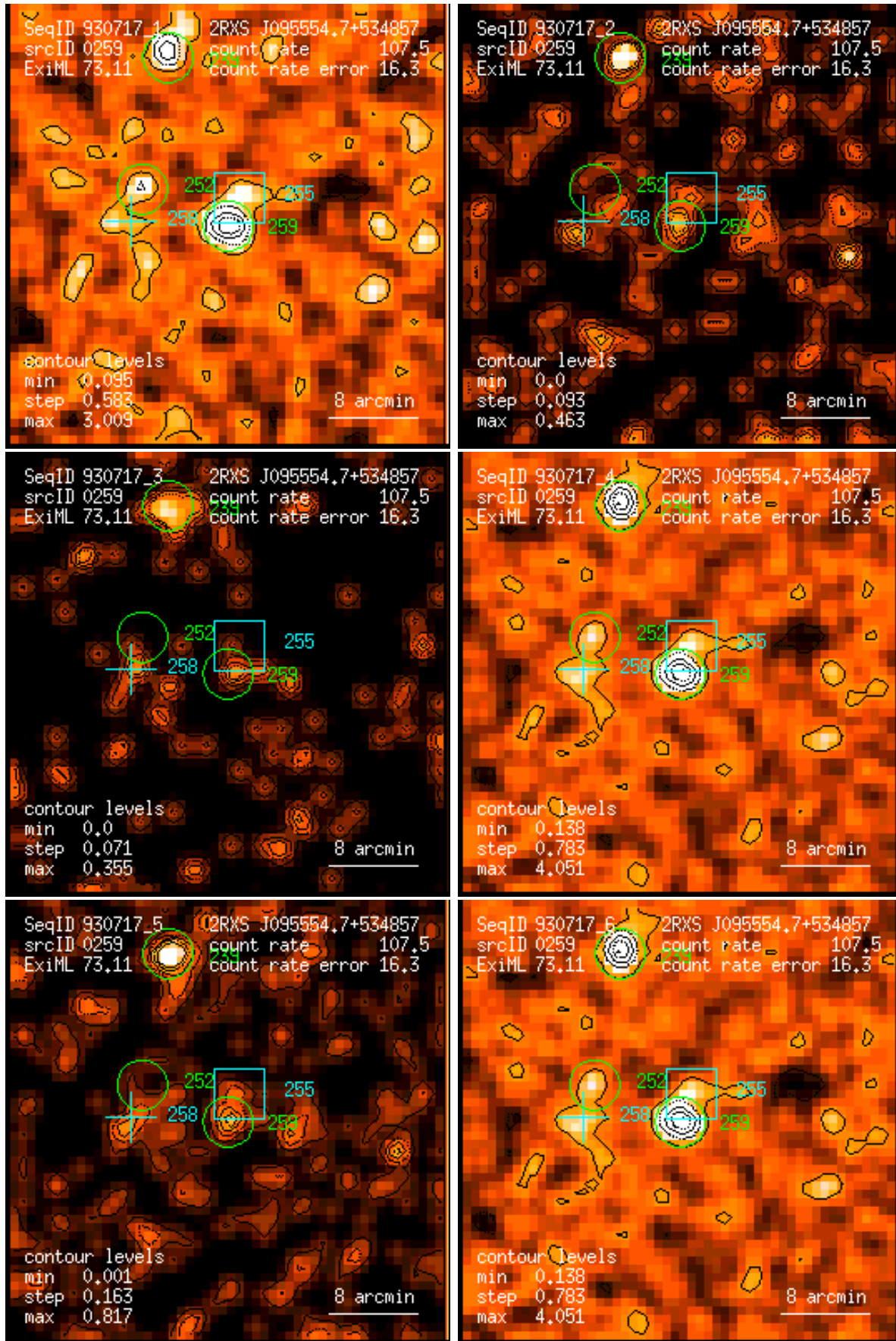
Figure 259: RASS 930717: detection 0259: band rate images, Gaussian filter: (1) PSPC channels 11 – 41, (2) 52 – 90, (3) 91 – 201, (4) 11 – 235, (5) 52 – 201, (6) 11 – 201. Broad band rates in counts/ks. Band rate contour levels in counts/ks/arcmin 2 .
