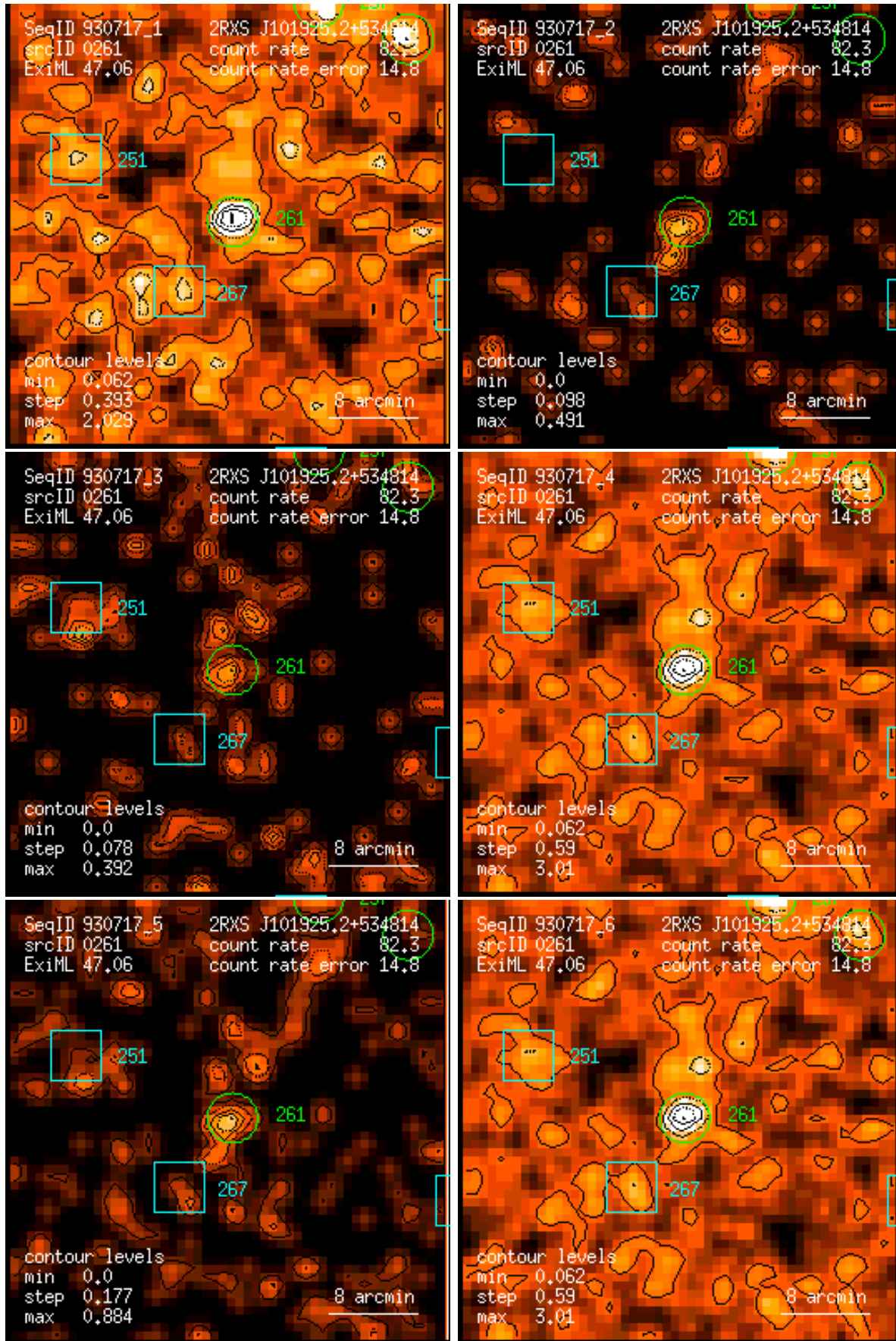
Figure 261: RASS 930717: detection 0261: band rate images, Gaussian filter: (1) PSPC channels 11 – 41, (2) 52 – 90, (3) 91 – 201, (4) 11 – 235, (5) 52 – 201, (6) 11 – 201. Broad band rates in counts/ks. Band rate contour levels in counts/ks/arcmin 2 .
