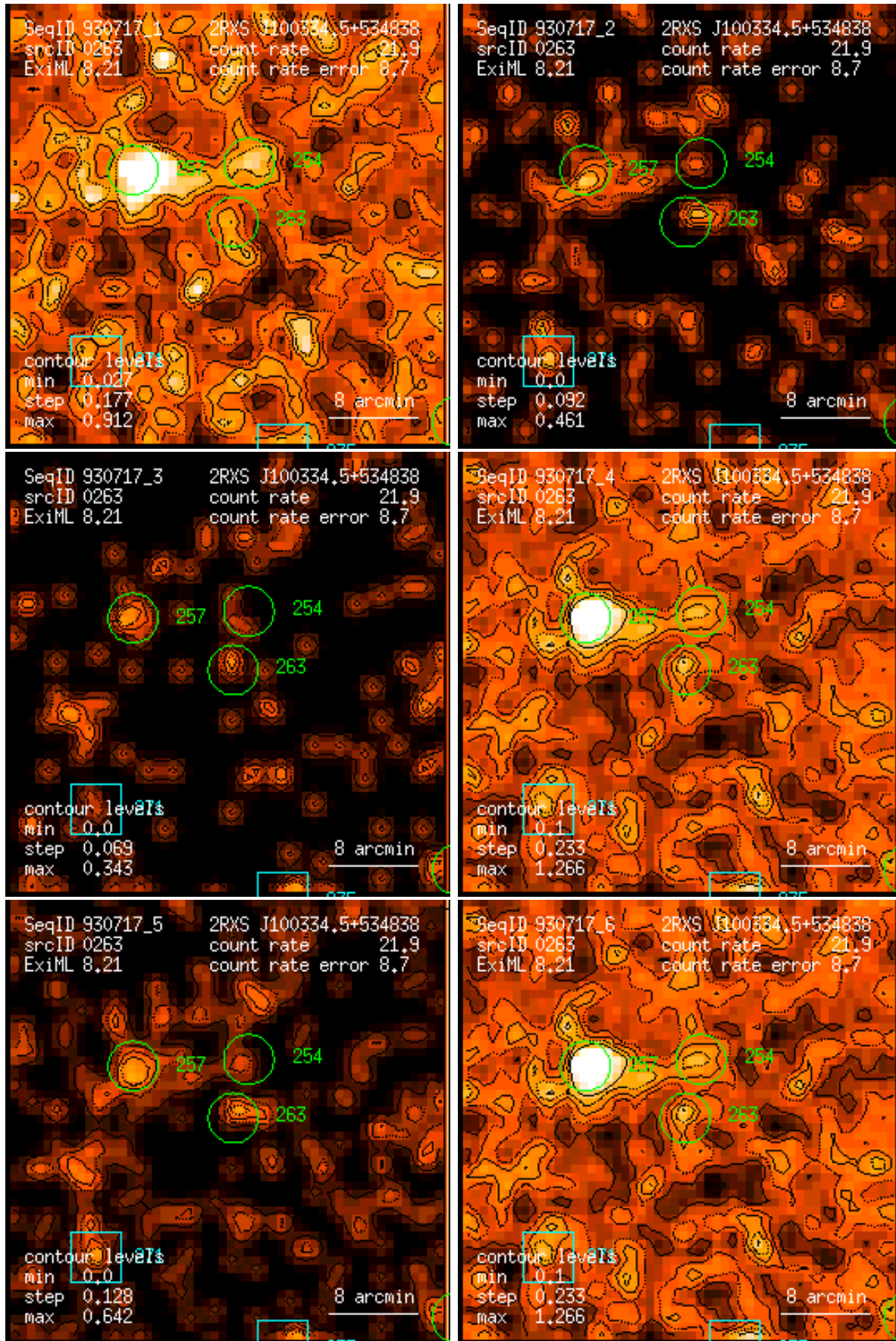
Figure 263: RASS 930717: detection 0263: band rate images, Gaussian filter: (1) PSPC channels 11 – 41, (2) 52 – 90, (3) 91 – 201, (4) 11 – 235, (5) 52 – 201, (6) 11 – 201. Broad band rates in counts/ks. Band rate contour levels in counts/ks/arcmin 2 .
