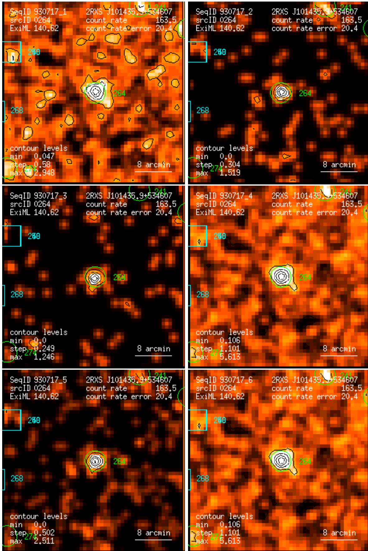
Figure 264: RASS 930717: detection 0264: band rate images, Gaussian filter: (1) PSPC channels 11 – 41, (2) 52 – 90, (3) 91 – 201, (4) 11 – 235, (5) 52 – 201, (6) 11 – 201. Broad band rates in counts/ks. Band rate contour levels in counts/ks/arcmin 2 .
