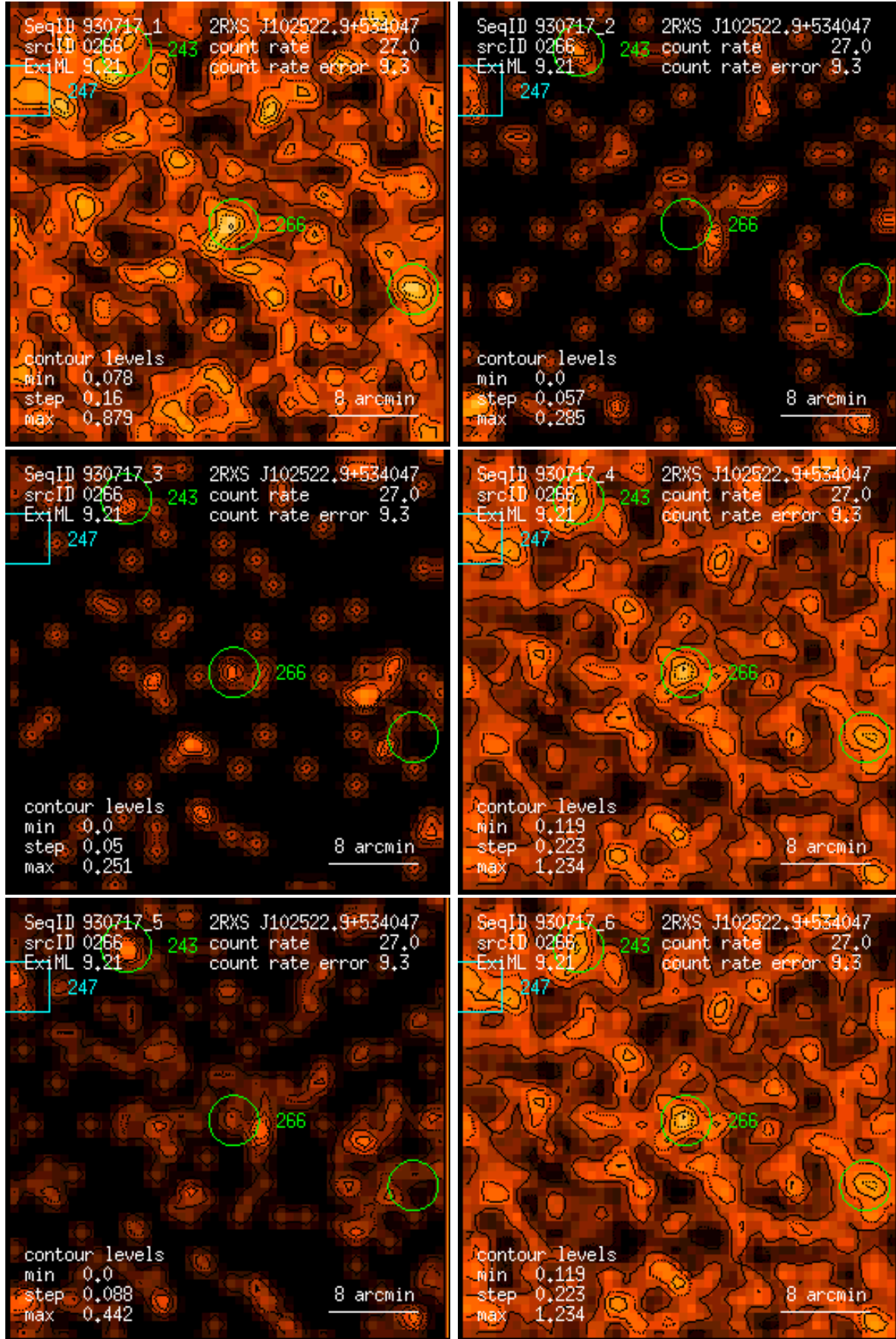
Figure 266: RASS 930717: detection 0266: band rate images, Gaussian filter: (1) PSPC channels 11 – 41, (2) 52 – 90, (3) 91 – 201, (4) 11 – 235, (5) 52 – 201, (6) 11 – 201. Broad band rates in counts/ks. Band rate contour levels in counts/ks/arcmin 2 .
