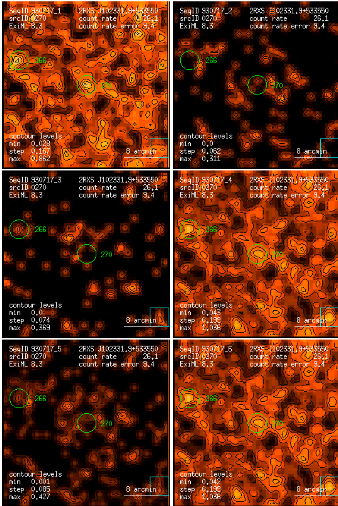
Figure 270: RASS 930717: detection 0270: band rate images, Gaussian filter: (1) PSPC channels 11 – 41, (2) 52 – 90, (3) 91 – 201, (4) 11 – 235, (5) 52 – 201, (6) 11 – 201. Broad band rates in counts/ks. Band rate contour levels in counts/ks/arcmin 2 .
