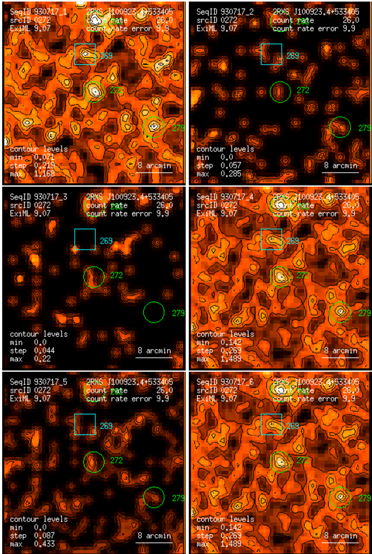
Figure 272: RASS 930717: detection 0272: band rate images, Gaussian filter: (1) PSPC channels 11 – 41, (2) 52 – 90, (3) 91 – 201, (4) 11 – 235, (5) 52 – 201, (6) 11 – 201. Broad band rates in counts/ks. Band rate contour levels in counts/ks/arcmin 2 .
