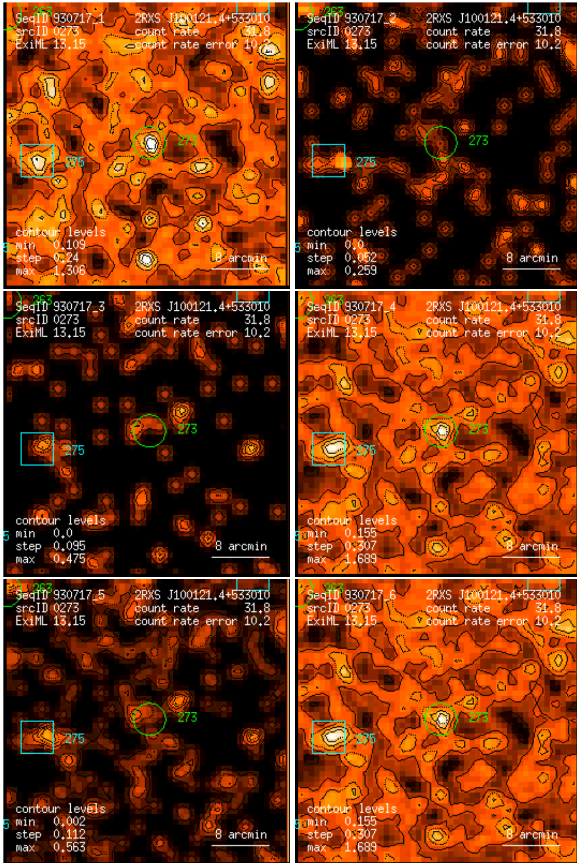
Figure 273: RASS 930717: detection 0273: band rate images, Gaussian filter: (1) PSPC channels 11 – 41, (2) 52 – 90, (3) 91 – 201, (4) 11 – 235, (5) 52 – 201, (6) 11 – 201. Broad band rates in counts/ks. Band rate contour levels in counts/ks/arcmin 2 .
