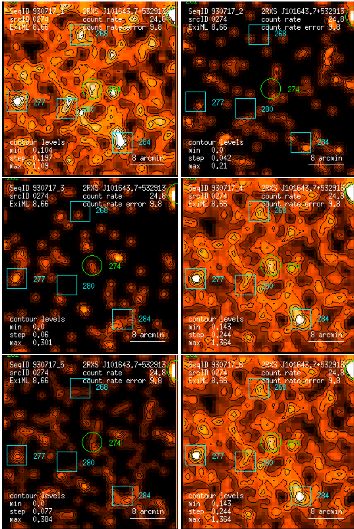
Figure 274: RASS 930717: detection 0274: band rate images, Gaussian filter: (1) PSPC channels 11 – 41, (2) 52 – 90, (3) 91 – 201, (4) 11 – 235, (5) 52 – 201, (6) 11 – 201. Broad band rates in counts/ks. Band rate contour levels in counts/ks/arcmin 2 .
