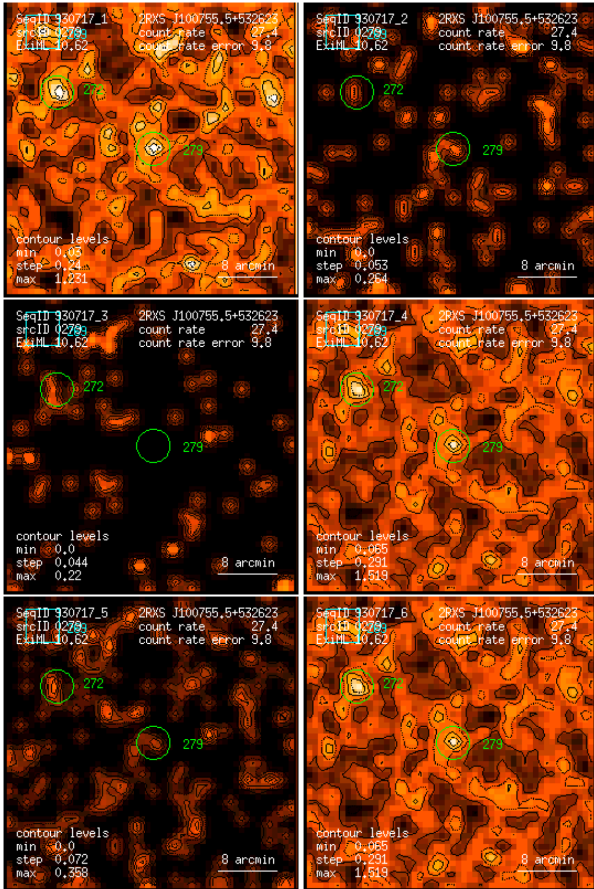
Figure 279: RASS 930717: detection 0279: band rate images, Gaussian filter: (1) PSPC channels 11 – 41, (2) 52 – 90, (3) 91 – 201, (4) 11 – 235, (5) 52 – 201, (6) 11 – 201. Broad band rates in counts/ks. Band rate contour levels in counts/ks/arcmin 2 .
