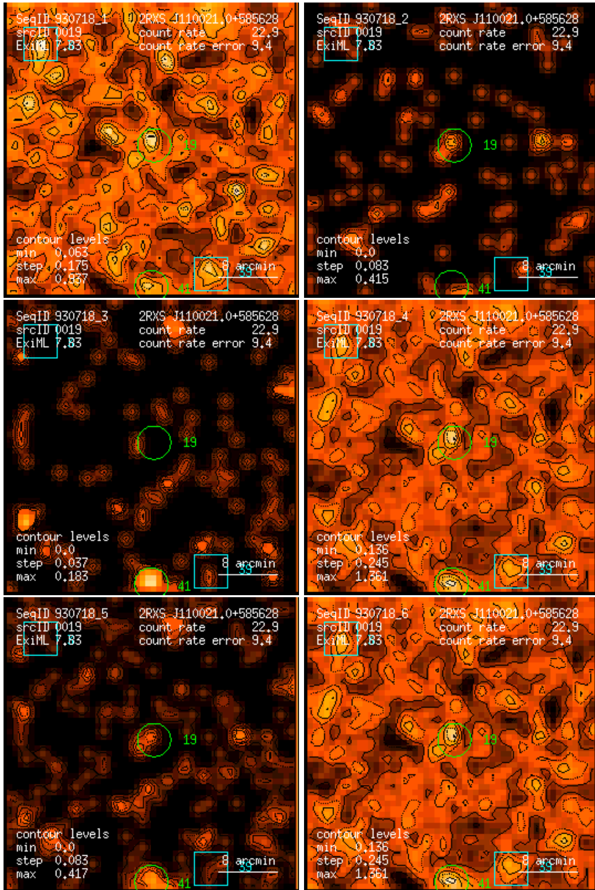
Figure 19: RASS 930718: detection 0019: band rate images, Gaussian filter: (1) PSPC channels 11 – 41, (2) 52 – 90, (3) 91 – 201, (4) 11 – 235, (5) 52 – 201, (6) 11 – 201. Broad band rates in counts/ks. Band rate contour levels in counts/ks/arcmin 2 .
