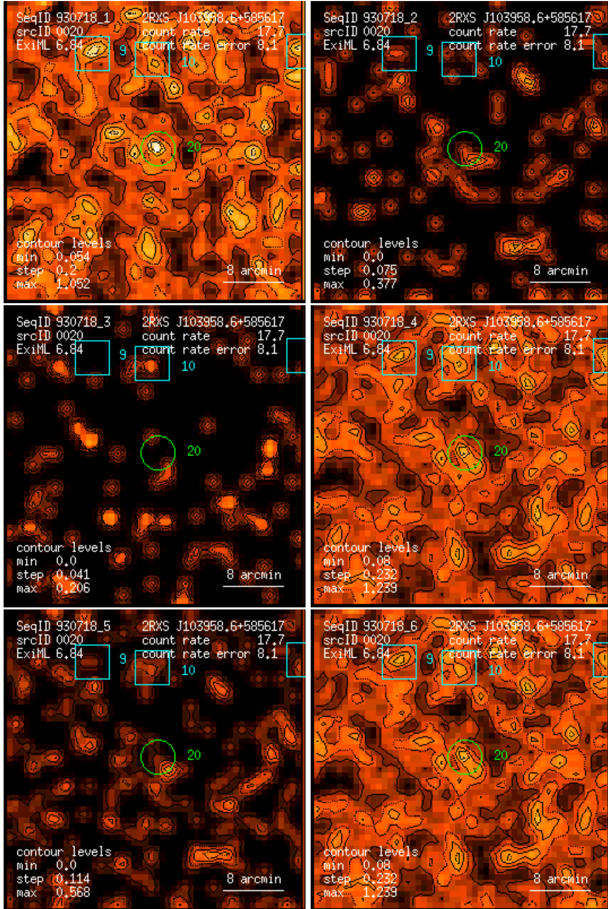
Figure 20: RASS 930718: detection 0020: band rate images, Gaussian filter: (1) PSPC channels 11 – 41, (2) 52 – 90, (3) 91 – 201, (4) 11 – 235, (5) 52 – 201, (6) 11 – 201. Broad band rates in counts/ks. Band rate contour levels in counts/ks/arcmin 2 .
