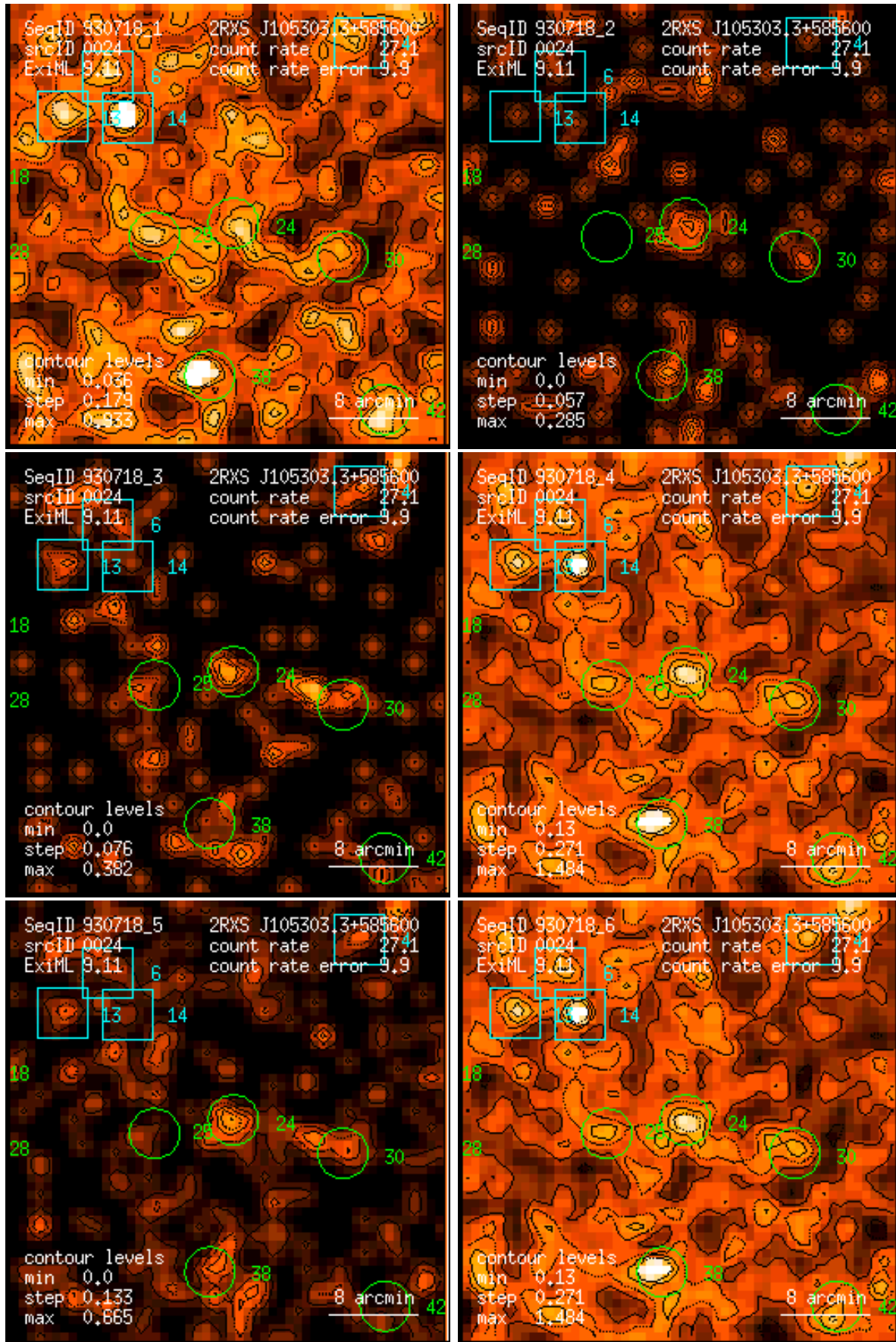
Figure 24: RASS 930718: detection 0024: band rate images, Gaussian filter: (1) PSPC channels 11 – 41, (2) 52 – 90, (3) 91 – 201, (4) 11 – 235, (5) 52 – 201, (6) 11 – 201. Broad band rates in counts/ks. Band rate contour levels in counts/ks/arcmin 2 .
