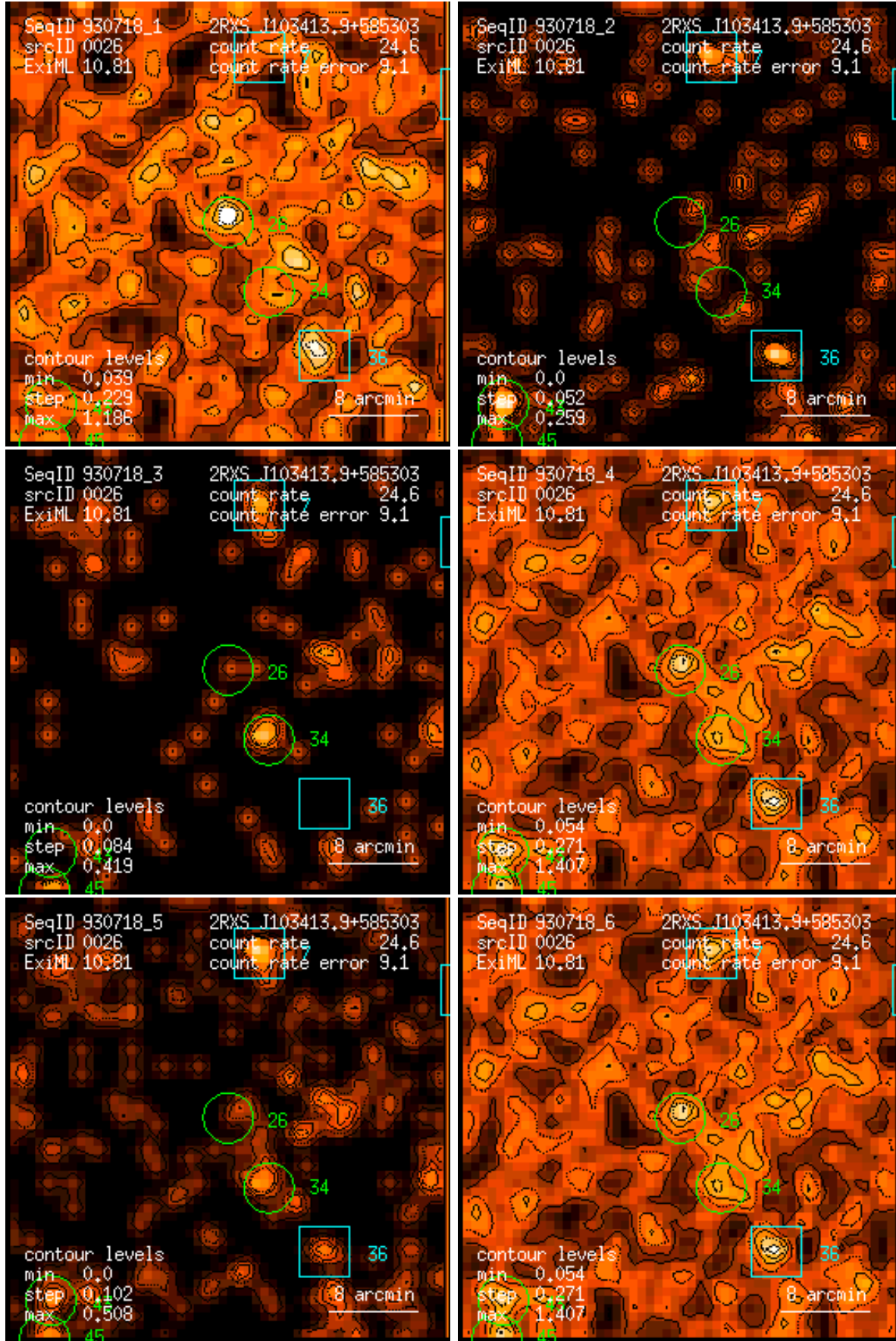
Figure 26: RASS 930718: detection 0026: band rate images, Gaussian filter: (1) PSPC channels 11 – 41, (2) 52 – 90, (3) 91 – 201, (4) 11 – 235, (5) 52 – 201, (6) 11 – 201. Broad band rates in counts/ks. Band rate contour levels in counts/ks/arcmin 2 .
