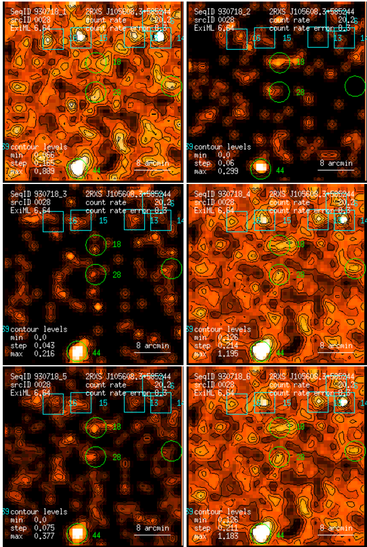
Figure 28: RASS 930718: detection 0028: band rate images, Gaussian filter: (1) PSPC channels 11 – 41, (2) 52 – 90, (3) 91 – 201, (4) 11 – 235, (5) 52 – 201, (6) 11 – 201. Broad band rates in counts/ks. Band rate contour levels in counts/ks/arcmin 2 .
