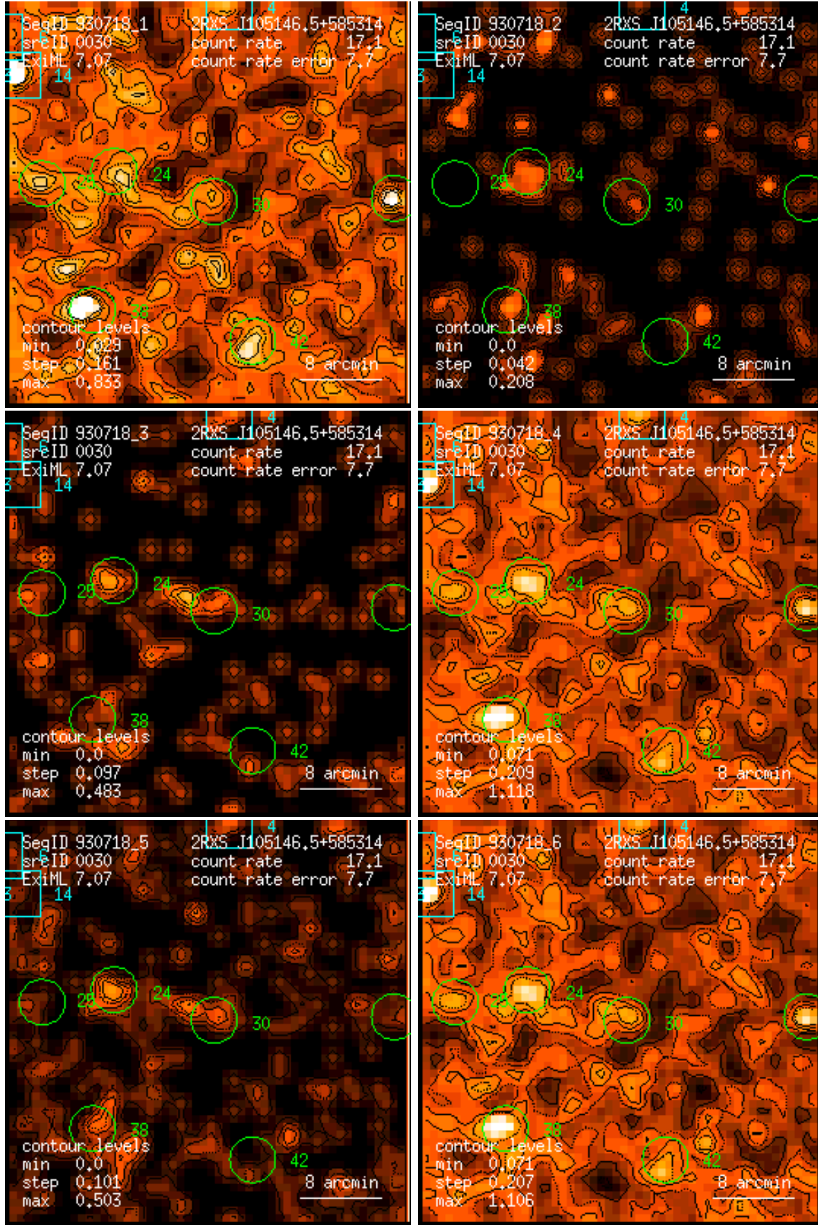
Figure 30: RASS 930718: detection 0030: band rate images, Gaussian filter: (1) PSPC channels 11 – 41, (2) 52 – 90, (3) 91 – 201, (4) 11 – 235, (5) 52 – 201, (6) 11 – 201. Broad band rates in counts/ks. Band rate contour levels in counts/ks/arcmin 2 .
