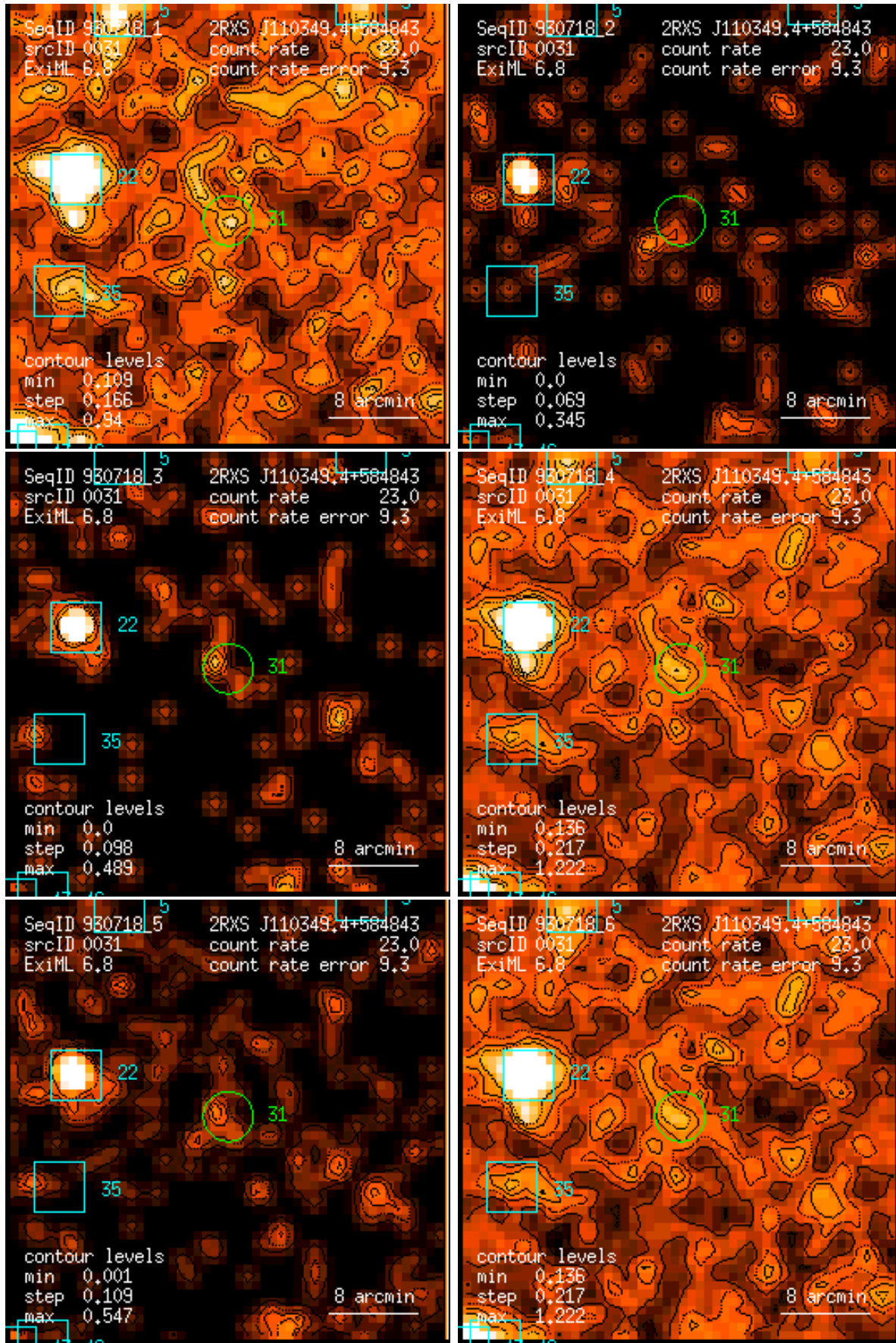
Figure 31: RASS 930718: detection 0031: band rate images, Gaussian filter: (1) PSPC channels 11 – 41, (2) 52 – 90, (3) 91 – 201, (4) 11 – 235, (5) 52 – 201, (6) 11 – 201. Broad band rates in counts/ks. Band rate contour levels in counts/ks/arcmin 2 .
