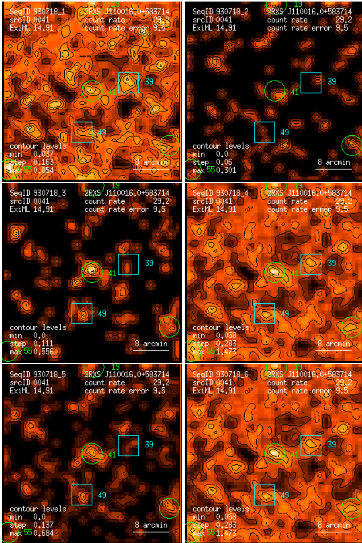
Figure 41: RASS 930718: detection 0041: band rate images, Gaussian filter: (1) PSPC channels 11 – 41, (2) 52 – 90, (3) 91 – 201, (4) 11 – 235, (5) 52 – 201, (6) 11 – 201. Broad band rates in counts/ks. Band rate contour levels in counts/ks/arcmin 2 .
