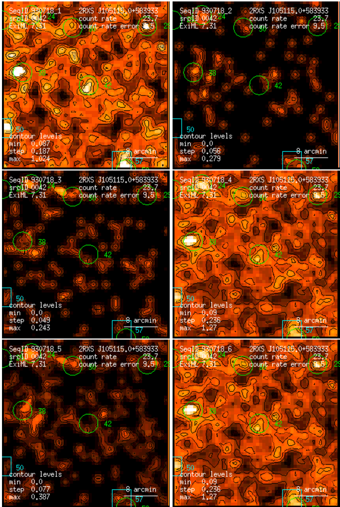
Figure 42: RASS 930718: detection 0042: band rate images, Gaussian filter: (1) PSPC channels 11 – 41, (2) 52 – 90, (3) 91 – 201, (4) 11 – 235, (5) 52 – 201, (6) 11 – 201. Broad band rates in counts/ks. Band rate contour levels in counts/ks/arcmin 2 .
