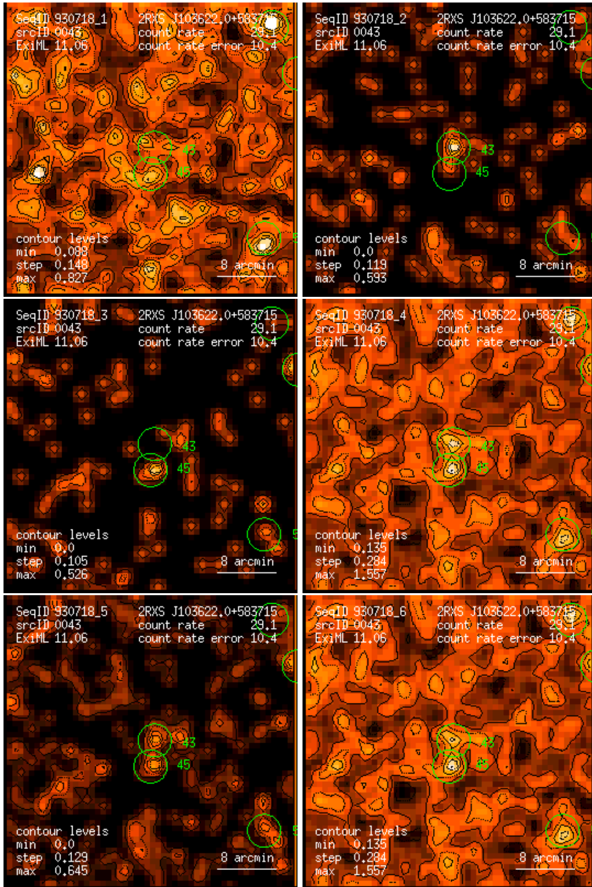
Figure 43: RASS 930718: detection 0043: band rate images, Gaussian filter: (1) PSPC channels 11 – 41, (2) 52 – 90, (3) 91 – 201, (4) 11 – 235, (5) 52 – 201, (6) 11 – 201. Broad band rates in counts/ks. Band rate contour levels in counts/ks/arcmin 2 .
