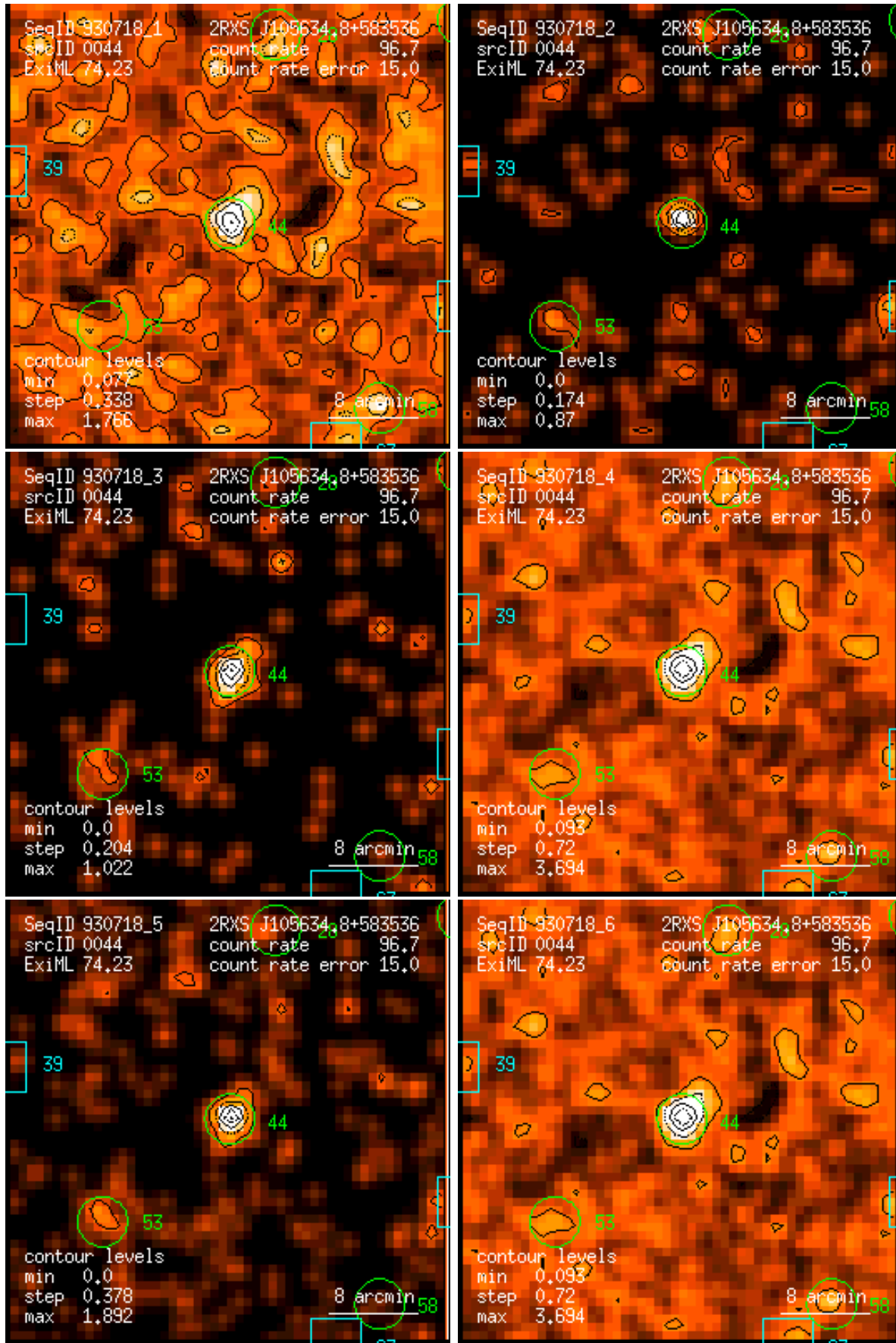
Figure 44: RASS 930718: detection 0044: band rate images, Gaussian filter: (1) PSPC channels 11 – 41, (2) 52 – 90, (3) 91 – 201, (4) 11 – 235, (5) 52 – 201, (6) 11 – 201. Broad band rates in counts/ks. Band rate contour levels in counts/ks/arcmin 2 .
