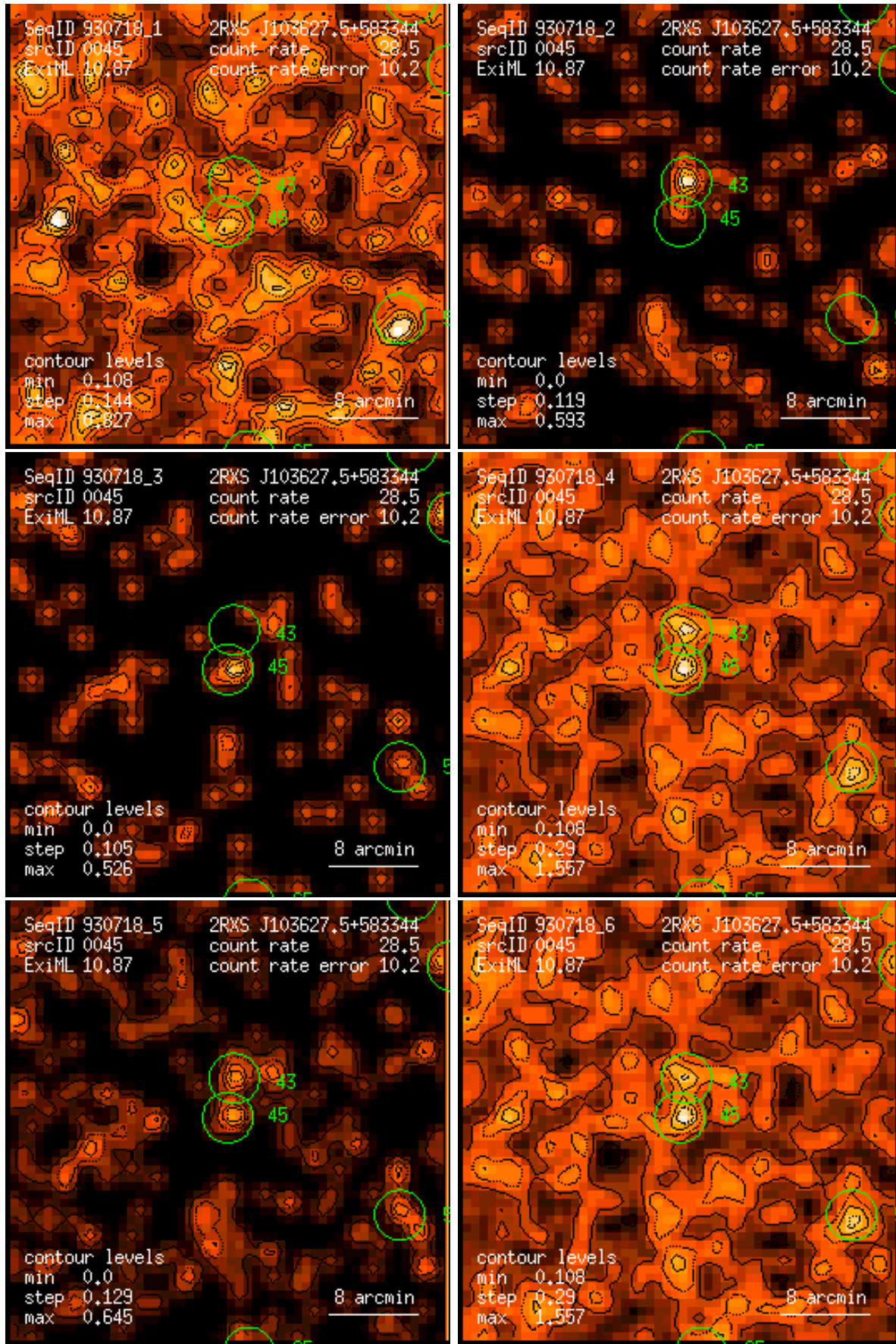
Figure 45: RASS 930718: detection 0045: band rate images, Gaussian filter: (1) PSPC channels 11 – 41, (2) 52 – 90, (3) 91 – 201, (4) 11 – 235, (5) 52 – 201, (6) 11 – 201. Broad band rates in counts/ks. Band rate contour levels in counts/ks/arcmin 2 .
