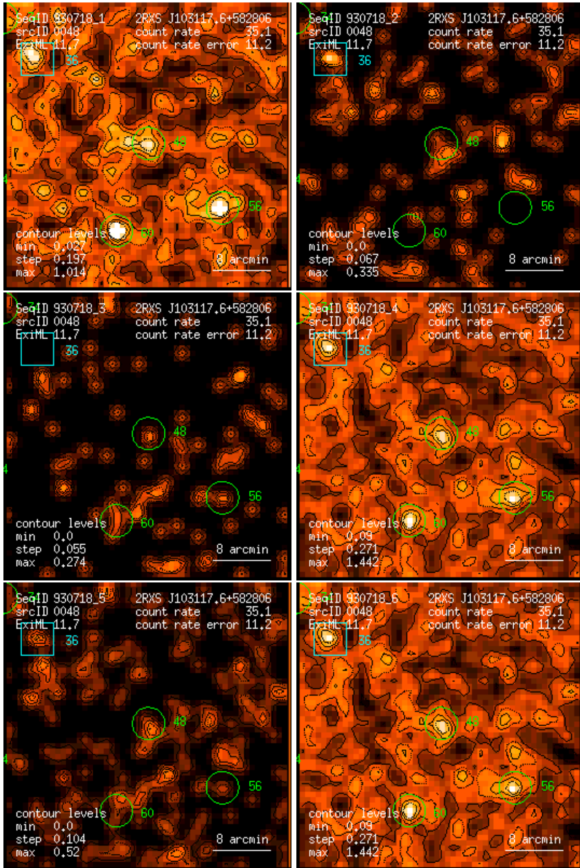
Figure 48: RASS 930718: detection 0048: band rate images, Gaussian filter: (1) PSPC channels 11 – 41, (2) 52 – 90, (3) 91 – 201, (4) 11 – 235, (5) 52 – 201, (6) 11 – 201. Broad band rates in counts/ks. Band rate contour levels in counts/ks/arcmin 2 .
