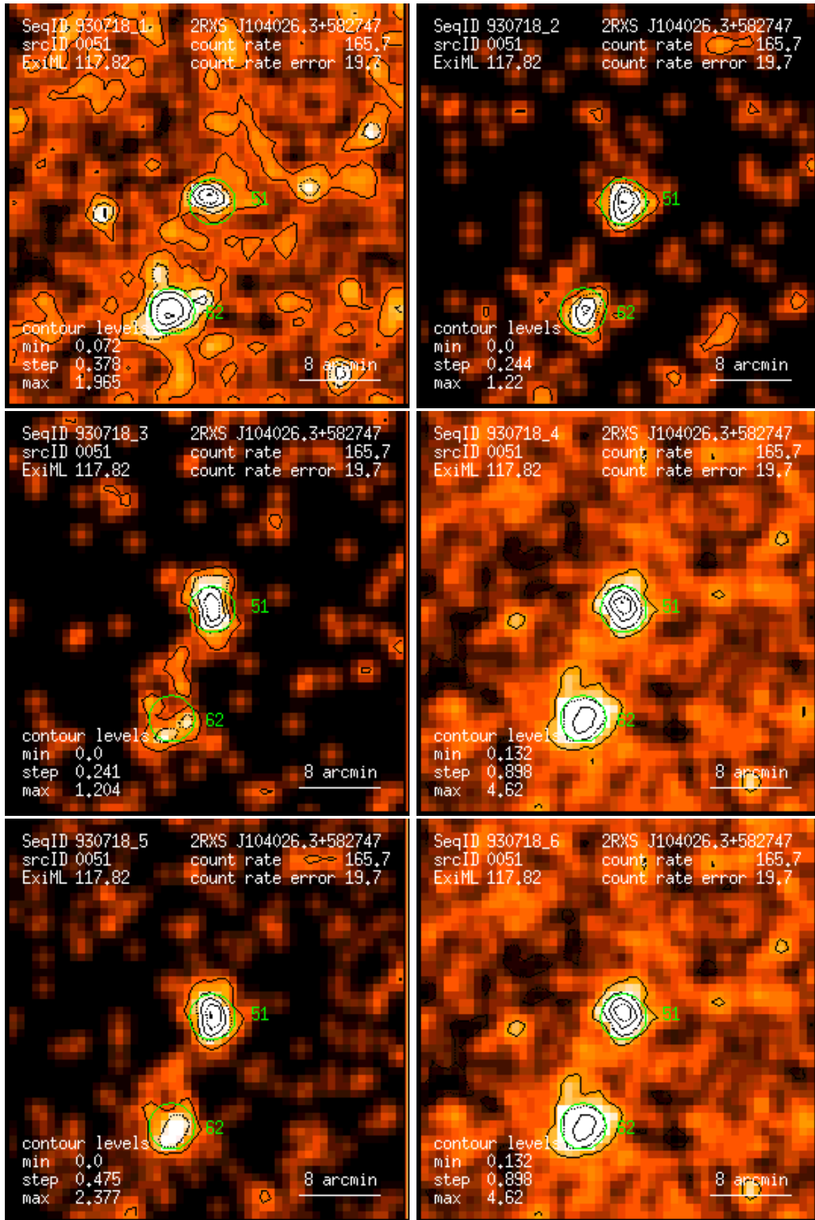
Figure 51: RASS 930718: detection 0051: band rate images, Gaussian filter: (1) PSPC channels 11 – 41, (2) 52 – 90, (3) 91 – 201, (4) 11 – 235, (5) 52 – 201, (6) 11 – 201. Broad band rates in counts/ks. Band rate contour levels in counts/ks/arcmin 2 .
