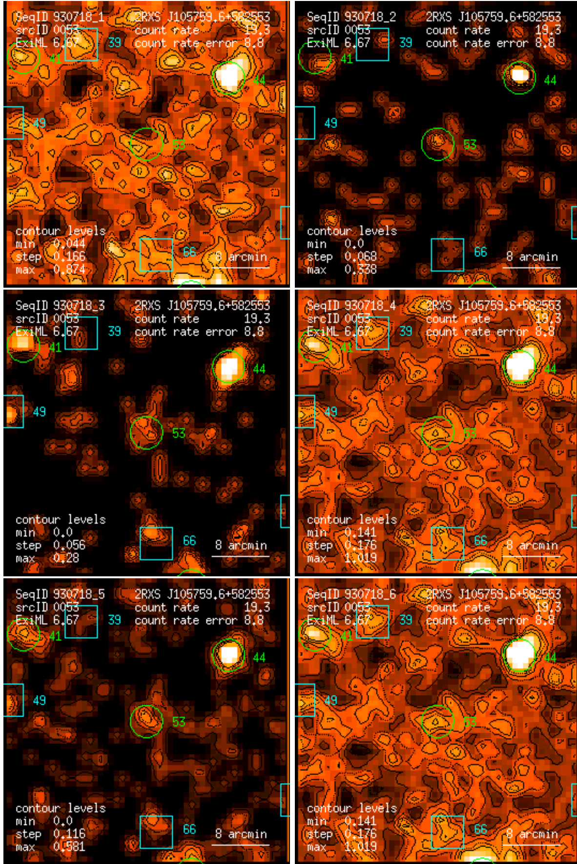
Figure 53: RASS 930718: detection 0053: band rate images, Gaussian filter: (1) PSPC channels 11 – 41, (2) 52 – 90, (3) 91 – 201, (4) 11 – 235, (5) 52 – 201, (6) 11 – 201. Broad band rates in counts/ks. Band rate contour levels in counts/ks/arcmin 2 .
