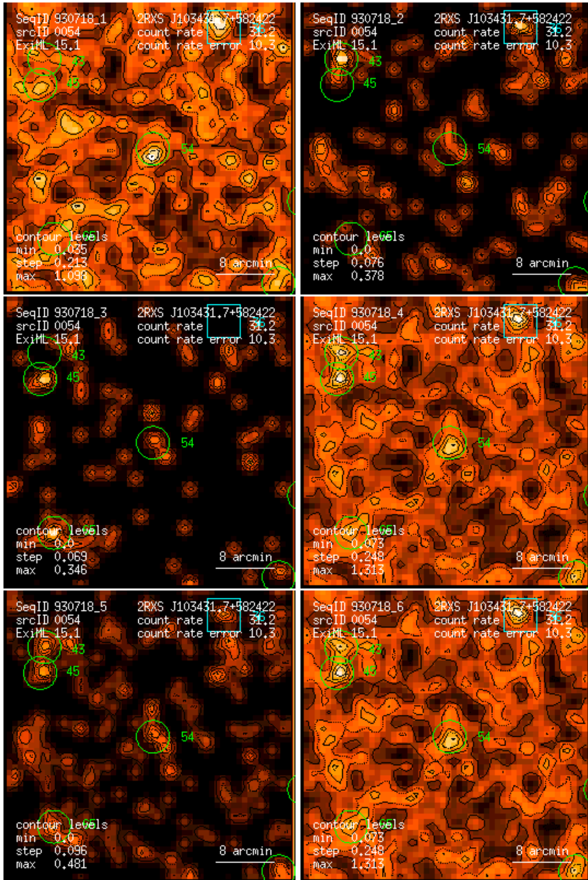
Figure 54: RASS 930718: detection 0054: band rate images, Gaussian filter: (1) PSPC channels 11 – 41, (2) 52 – 90, (3) 91 – 201, (4) 11 – 235, (5) 52 – 201, (6) 11 – 201. Broad band rates in counts/ks. Band rate contour levels in counts/ks/arcmin 2 .
