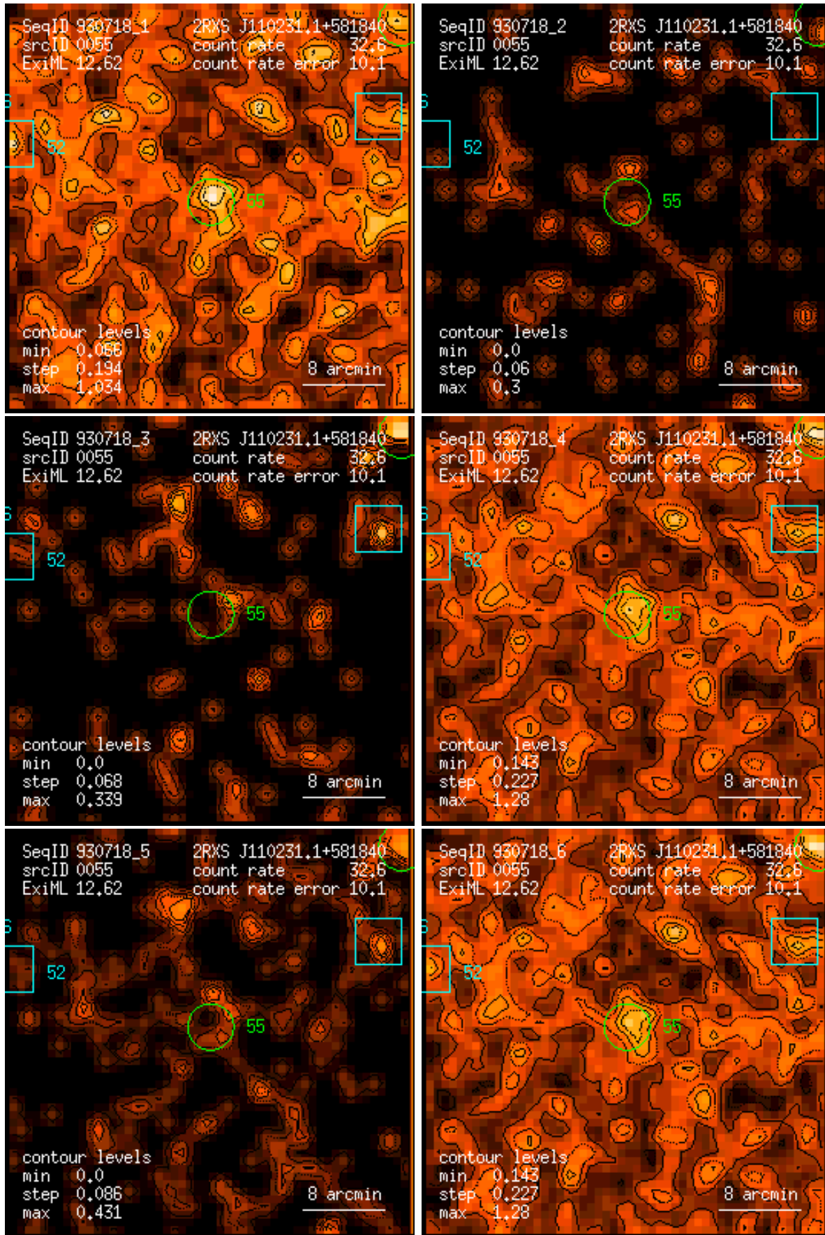
Figure 55: RASS 930718: detection 0055: band rate images, Gaussian filter: (1) PSPC channels 11 – 41, (2) 52 – 90, (3) 91 – 201, (4) 11 – 235, (5) 52 – 201, (6) 11 – 201. Broad band rates in counts/ks. Band rate contour levels in counts/ks/arcmin 2 .
