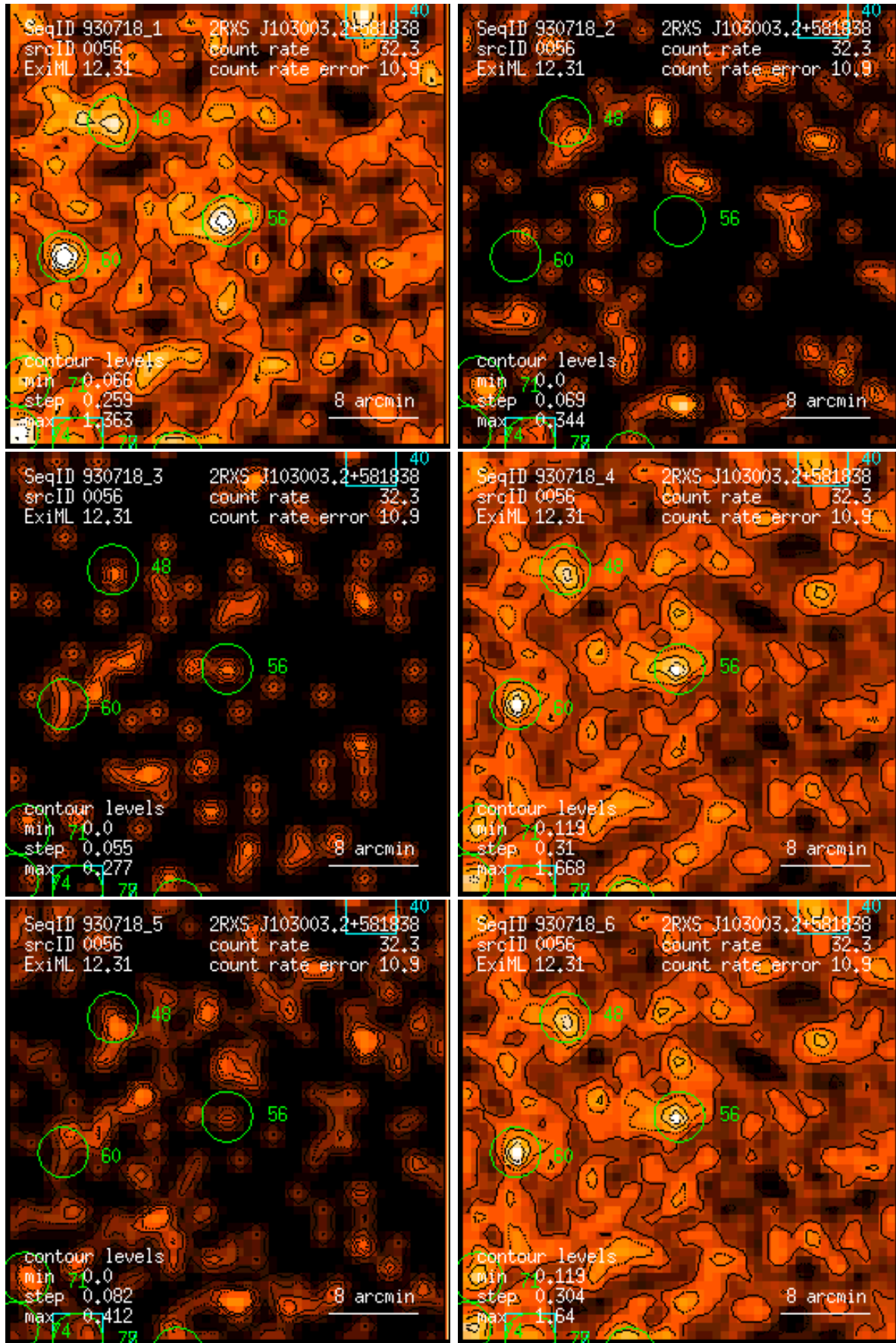
Figure 56: RASS 930718: detection 0056: band rate images, Gaussian filter: (1) PSPC channels 11 – 41, (2) 52 – 90, (3) 91 – 201, (4) 11 – 235, (5) 52 – 201, (6) 11 – 201. Broad band rates in counts/ks. Band rate contour levels in counts/ks/arcmin 2 .
