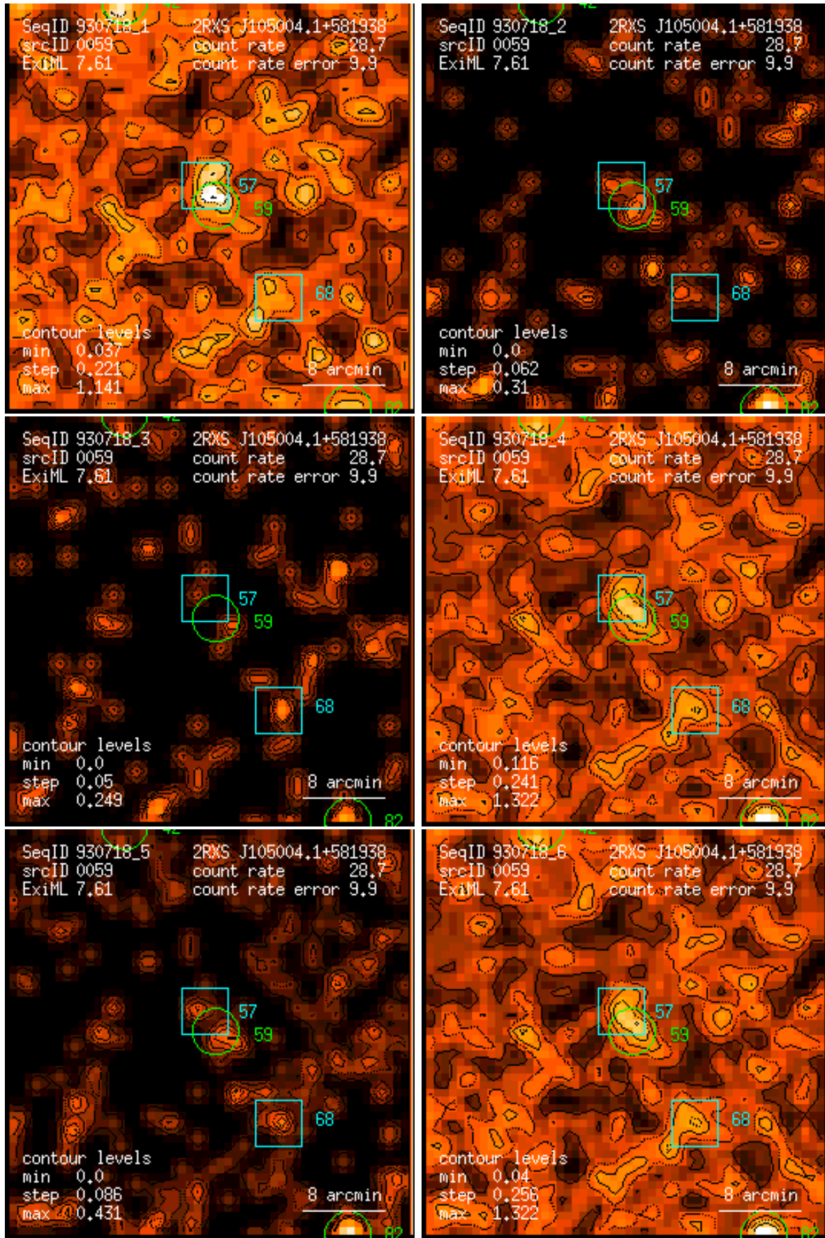
Figure 59: RASS 930718: detection 0059: band rate images, Gaussian filter: (1) PSPC channels 11 – 41, (2) 52 – 90, (3) 91 – 201, (4) 11 – 235, (5) 52 – 201, (6) 11 – 201. Broad band rates in counts/ks. Band rate contour levels in counts/ks/arcmin 2 .
