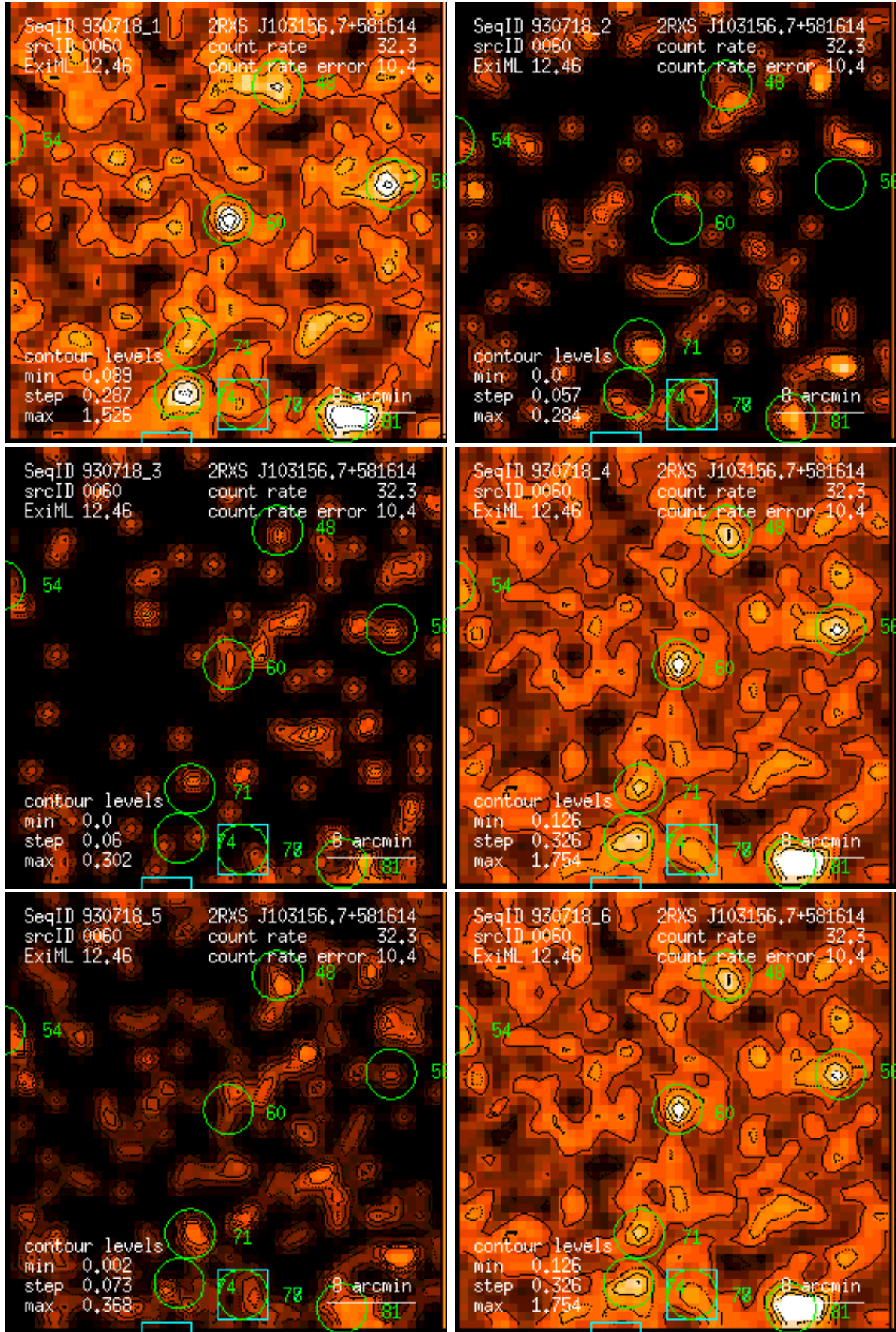
Figure 60: RASS 930718: detection 0060: band rate images, Gaussian filter: (1) PSPC channels 11 – 41, (2) 52 – 90, (3) 91 – 201, (4) 11 – 235, (5) 52 – 201, (6) 11 – 201. Broad band rates in counts/ks. Band rate contour levels in counts/ks/arcmin 2 .
